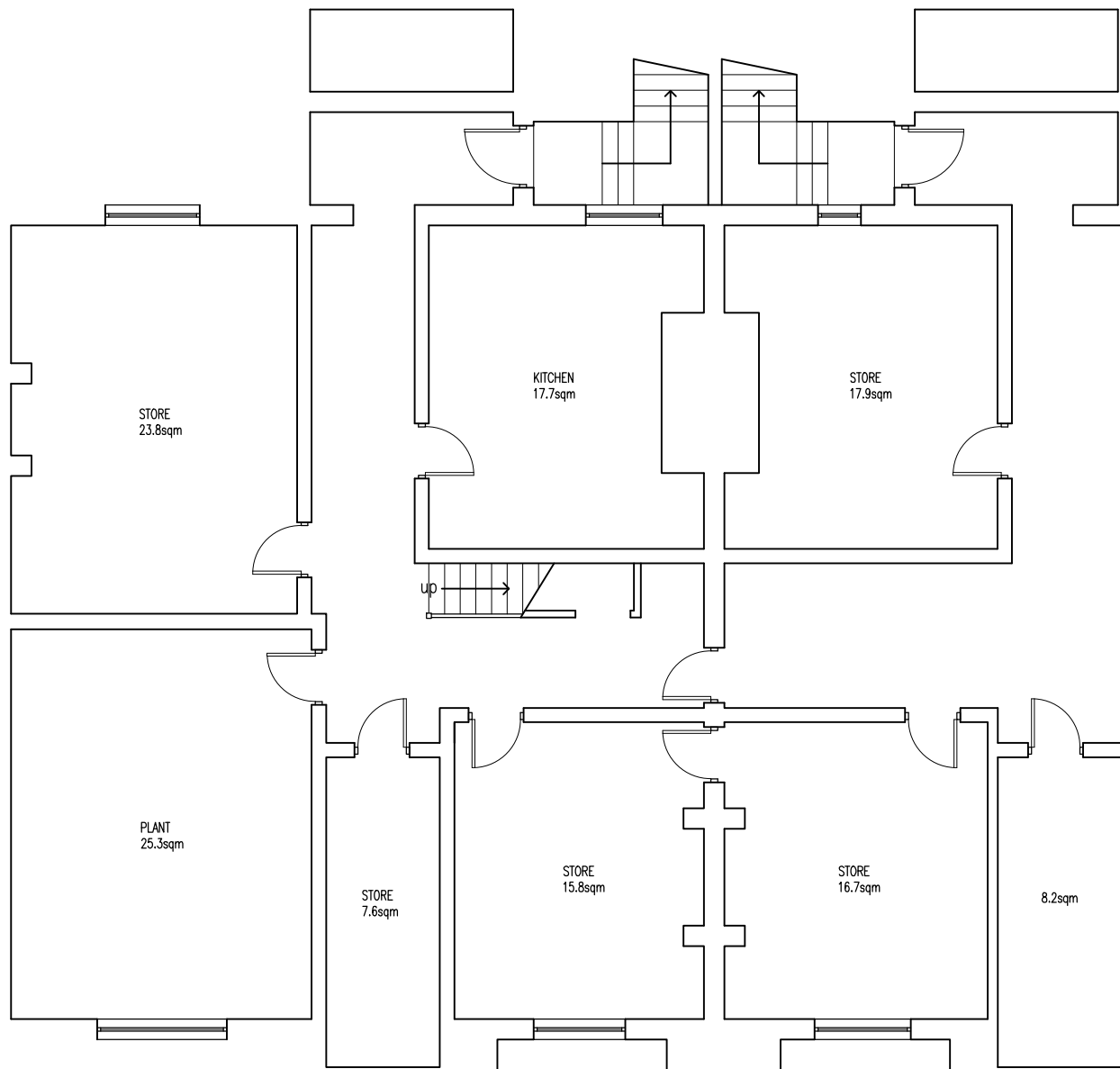
EXISTING BASEMENT FLOOR PLAN 1:100 @ A3
