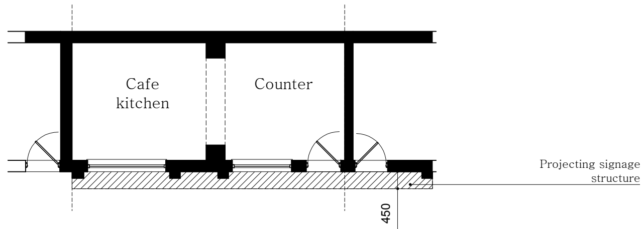
EXISTING FLOOR PLAN 1:100 (Pre development)
