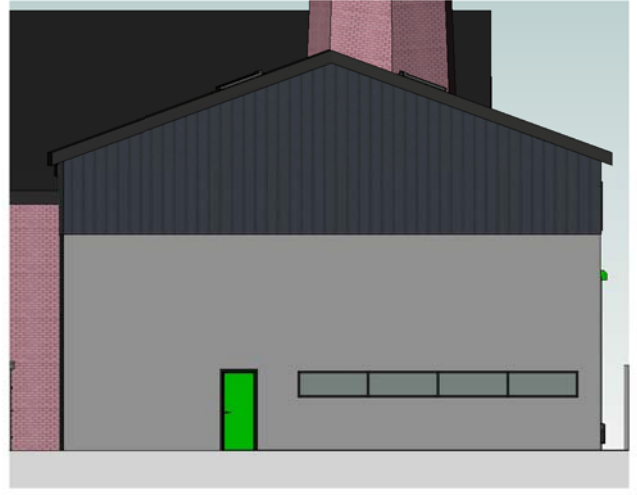
Unit 2 D - Side Elevation 1 : 200
