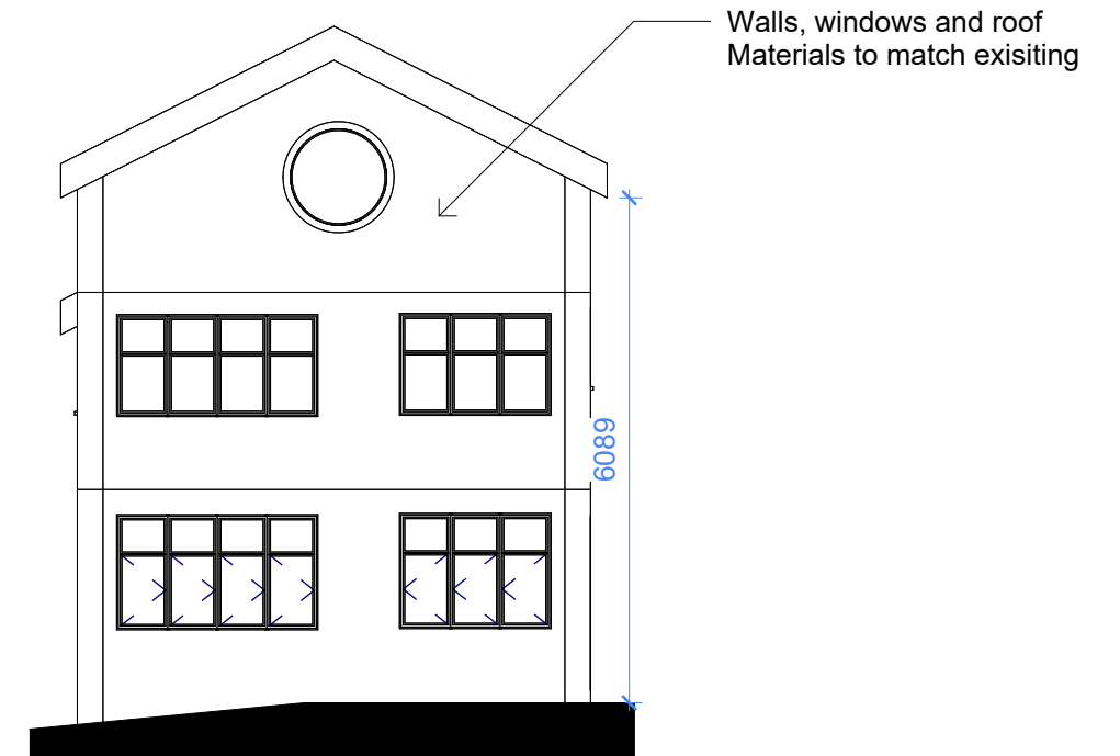
North Front -Proposed 1 : 100
