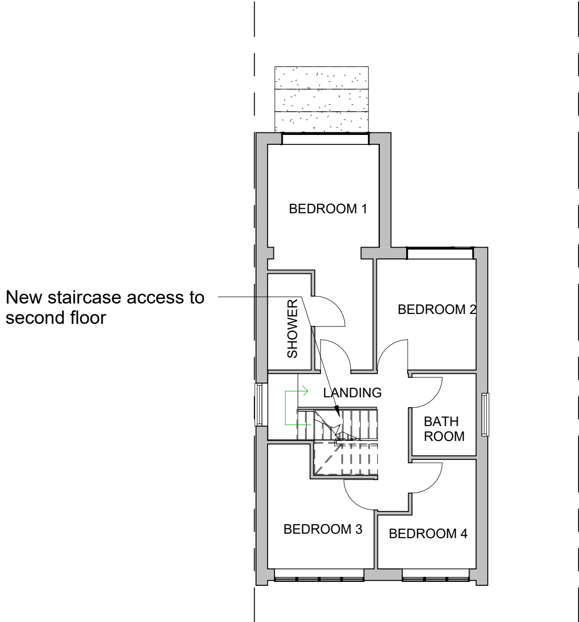
01 First floor-Proposed 1 : 100
