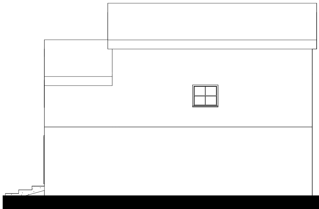
East -side -Proposed 1 : 100
