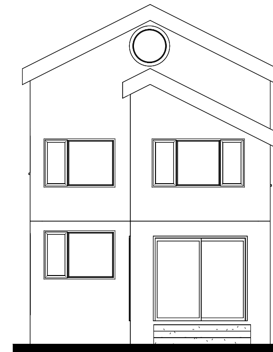
South- Rear -Proposed 1 : 100
