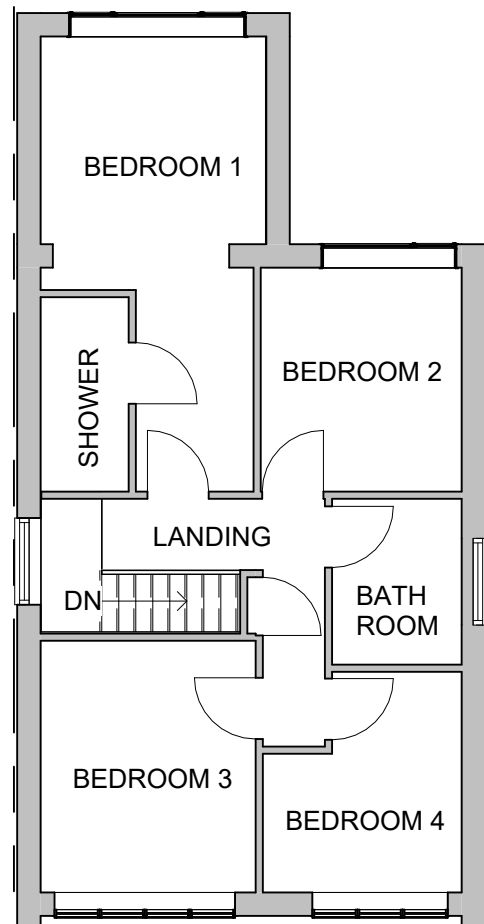
01 First floor 1 : 100
