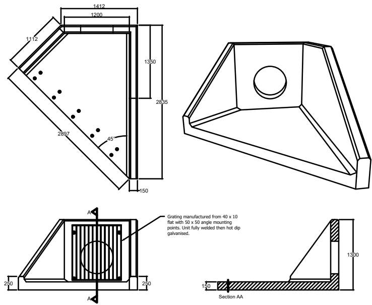
HEADWALL OUTLET 2 DETAIL (1:50)
