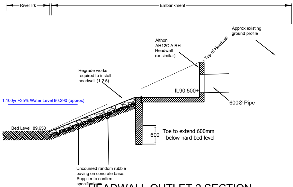
HEADWALL OUTLET 2 SECTION (1:50)
