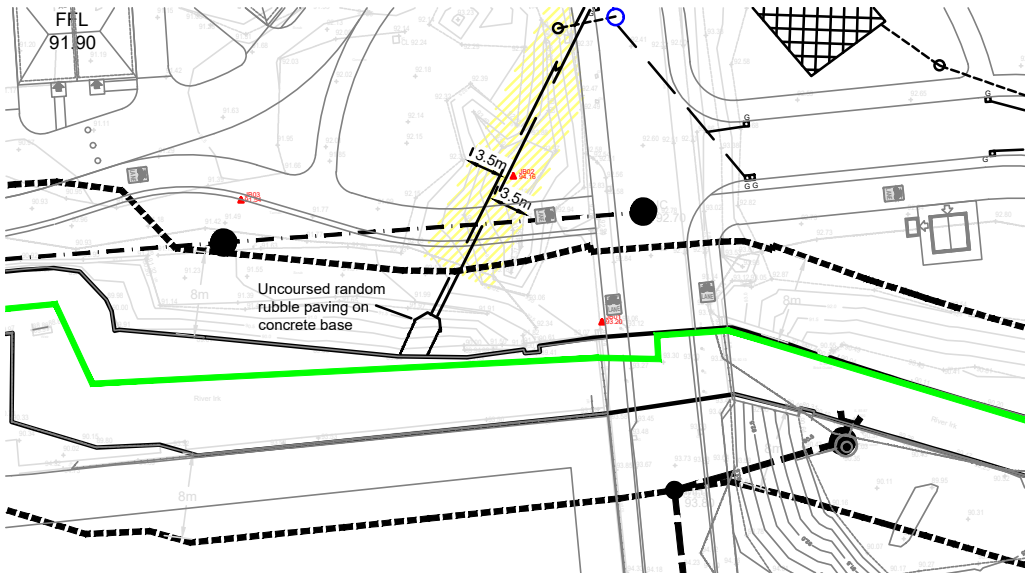
HEADWALL OUTLET 2 LOCATION PLAN (1:500)
