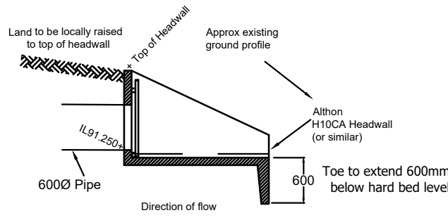
HEADWALL OUTLET 1 SECTION (1:50)
