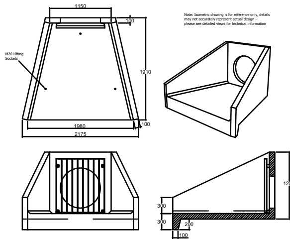
HEADWALL OUTLET 1 DETAIL (1:50)
