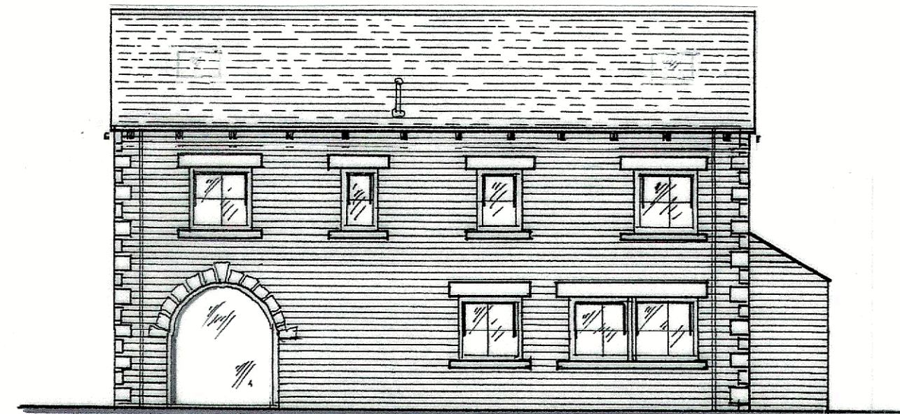
SOUTH ELEVATION.
