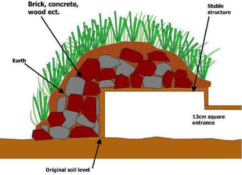
Typical Hedgehog Hibernacula Detail
