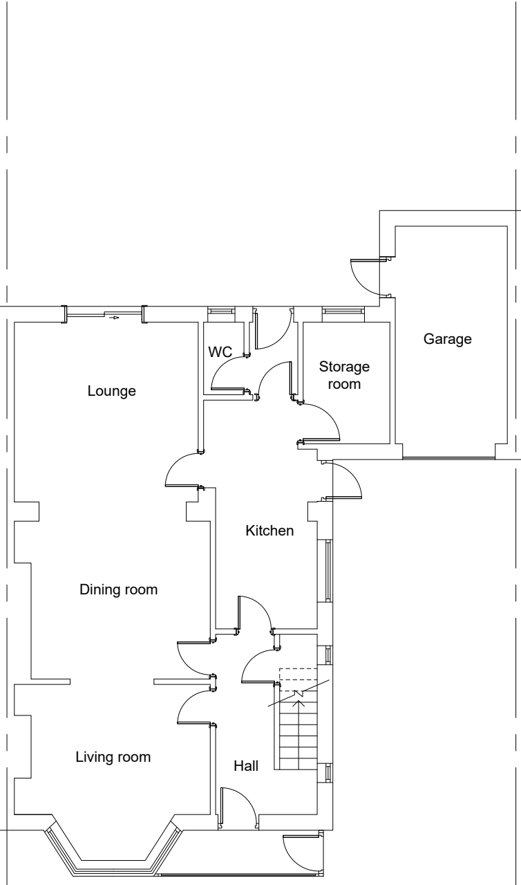
GROUND FLOOR PLAN (EXISTING)
