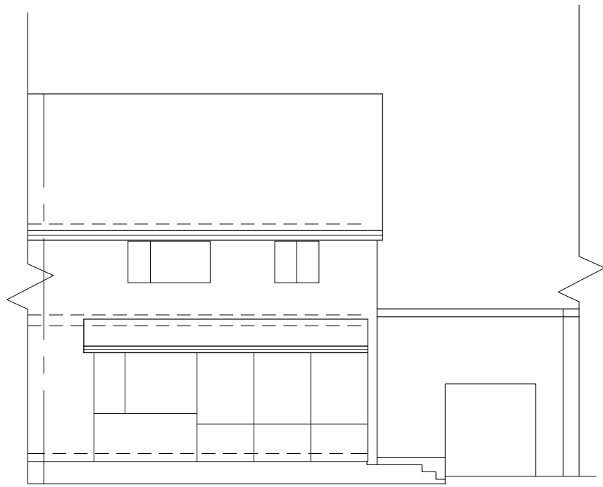
FRONT ELEVATION (EXISTING)
