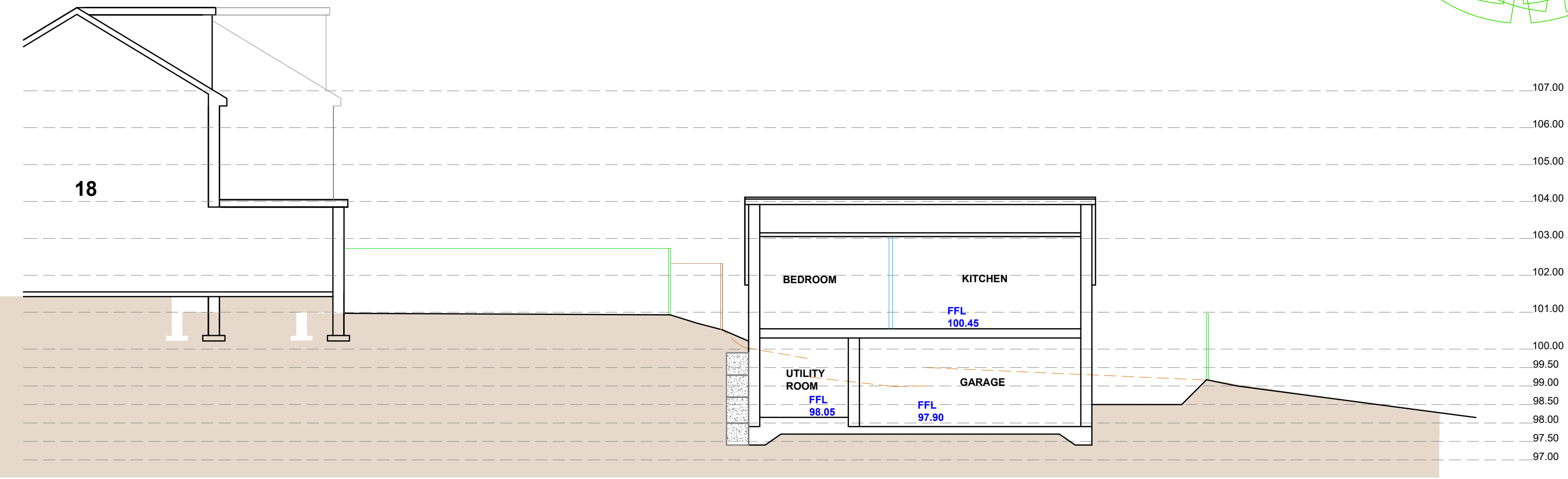
PROPOSED SECTION 2 - 2
