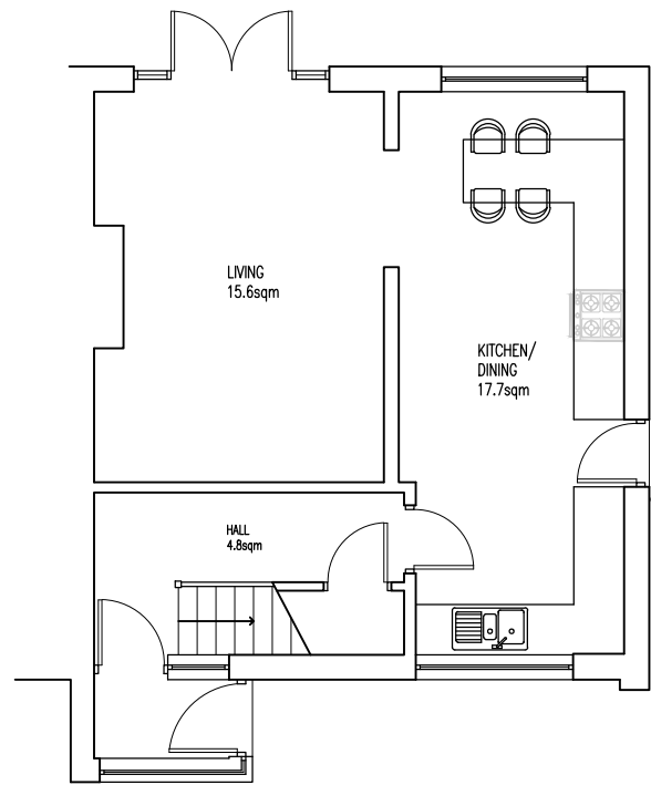
EXISTING GROUND FLOOR PLAN 1:100 @ A3
