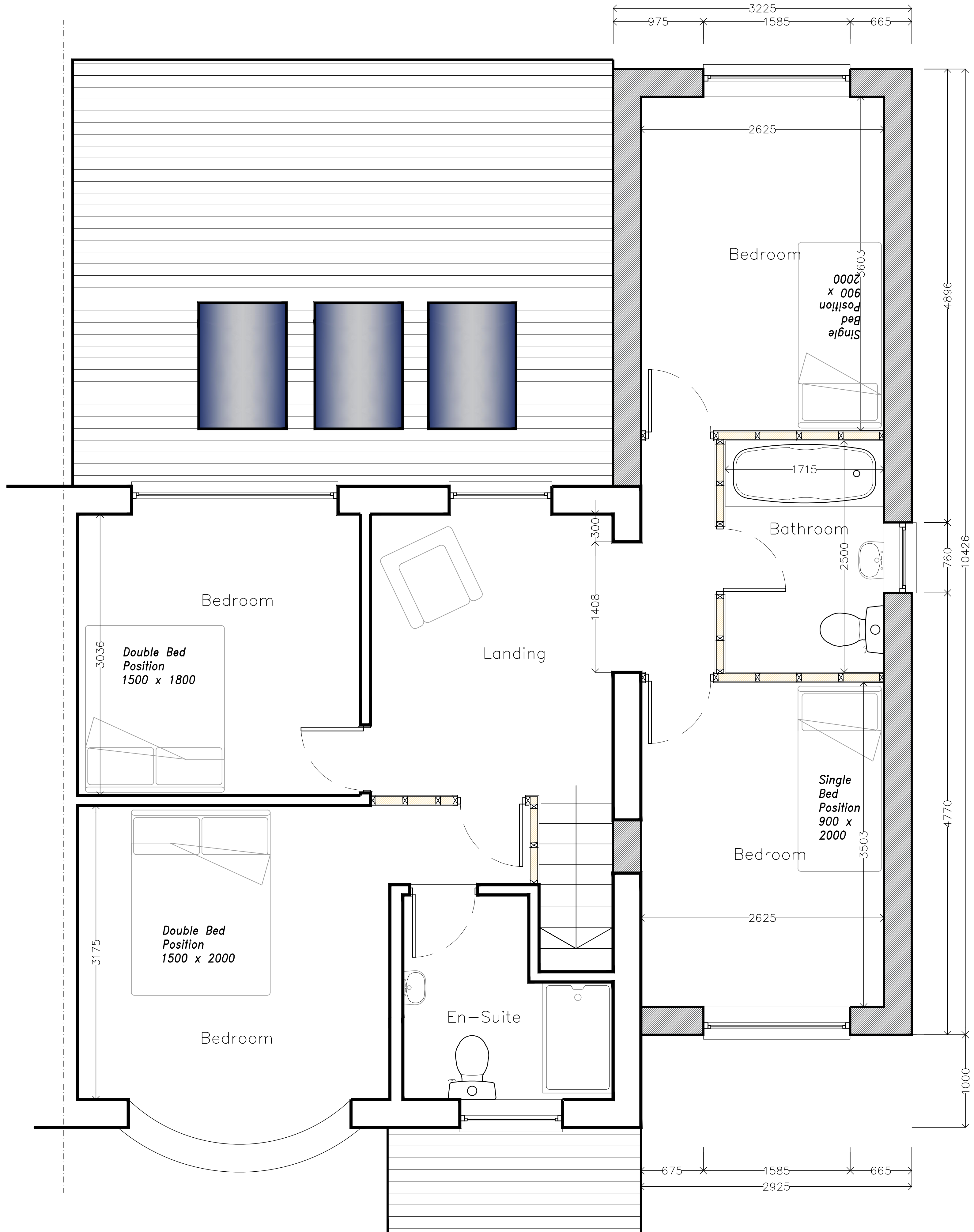
Proposed First Floor Plan (1:25)
