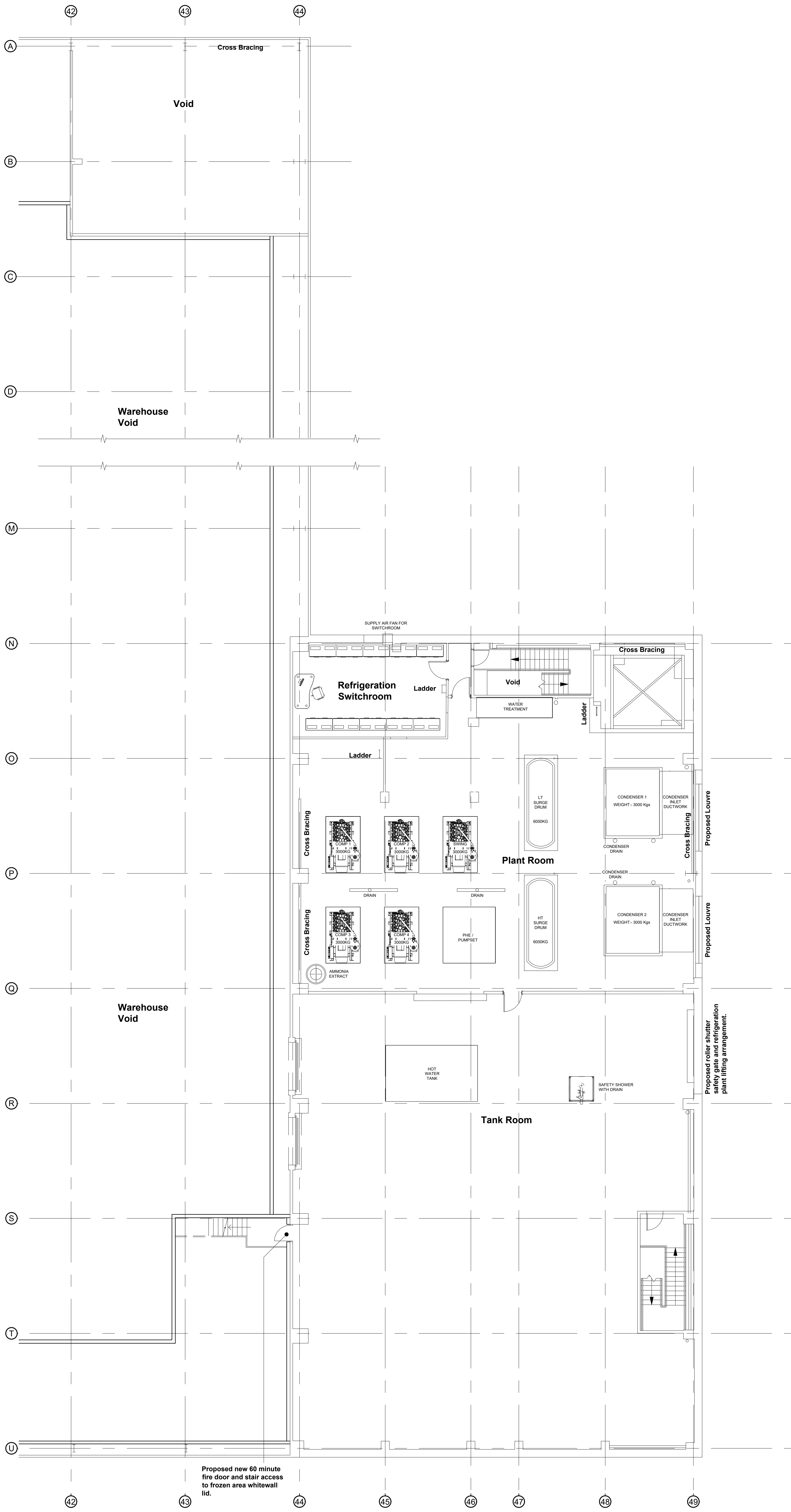
Proposed South Store - First Floor Scale 1:100
