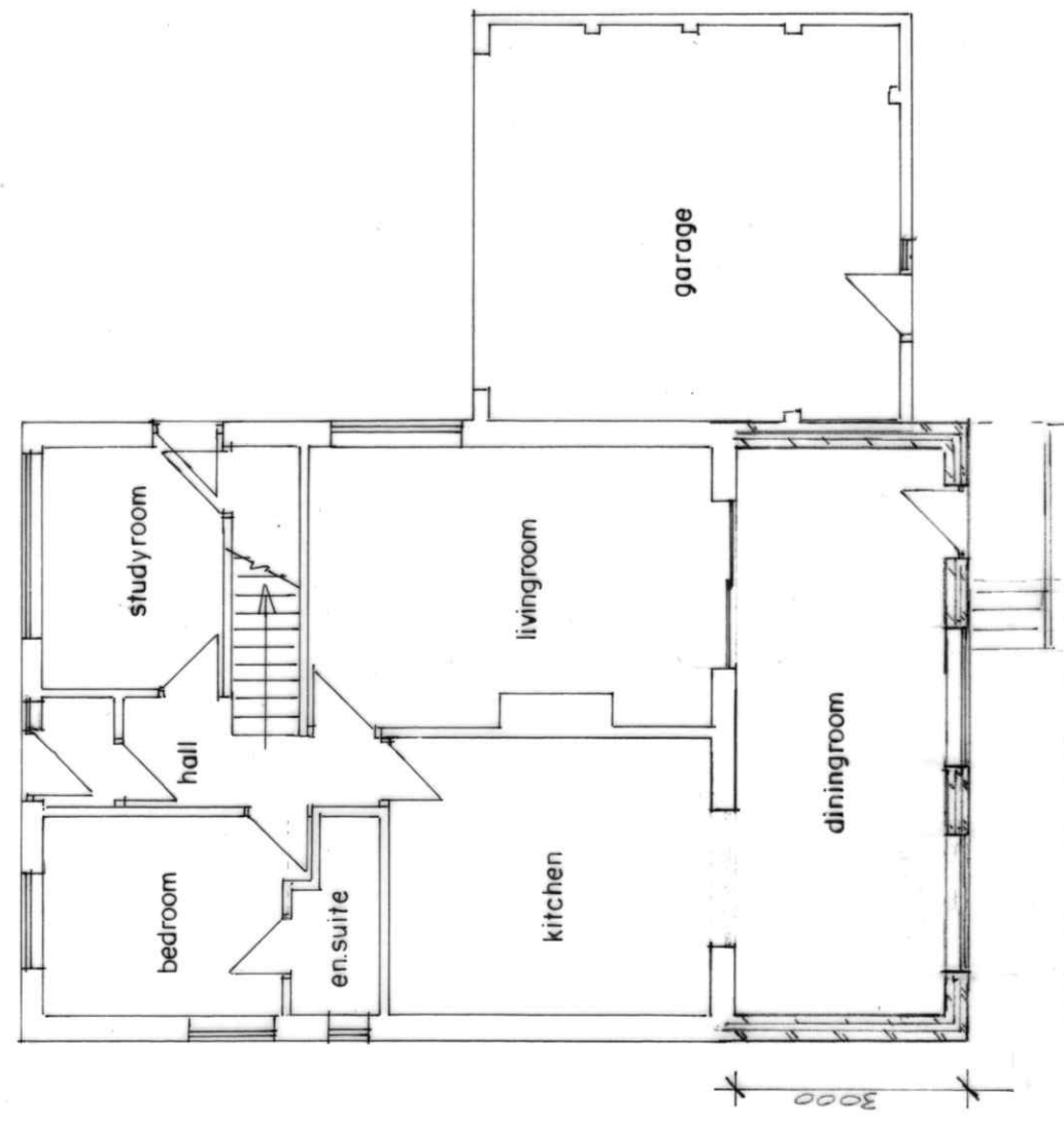
GROUND FLOOR PLAN (PROPOSED)
