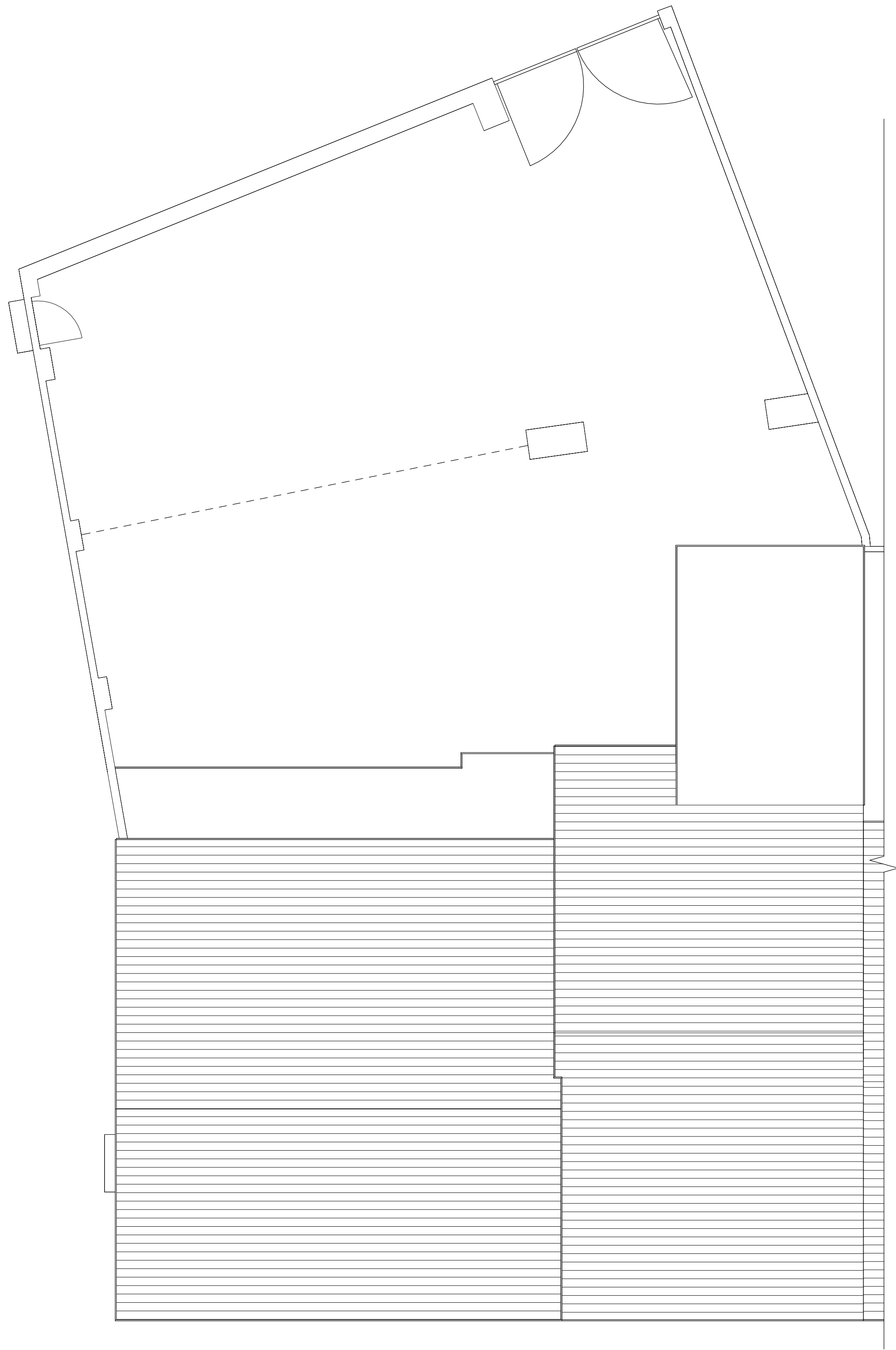
2 Level Roof - Existing 1 : 50
