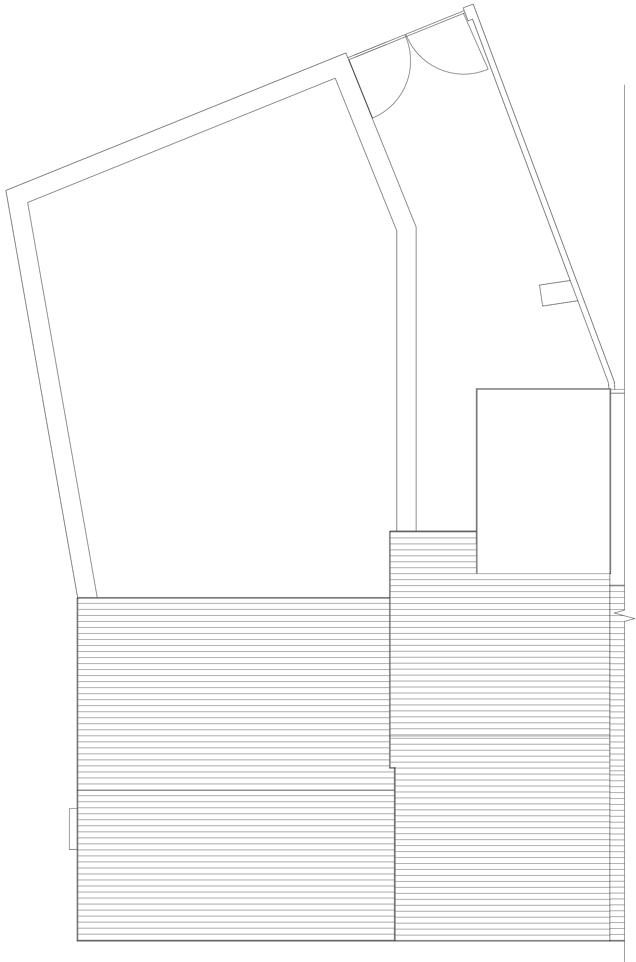
1 Level Roof - Proposed 1 : 50
