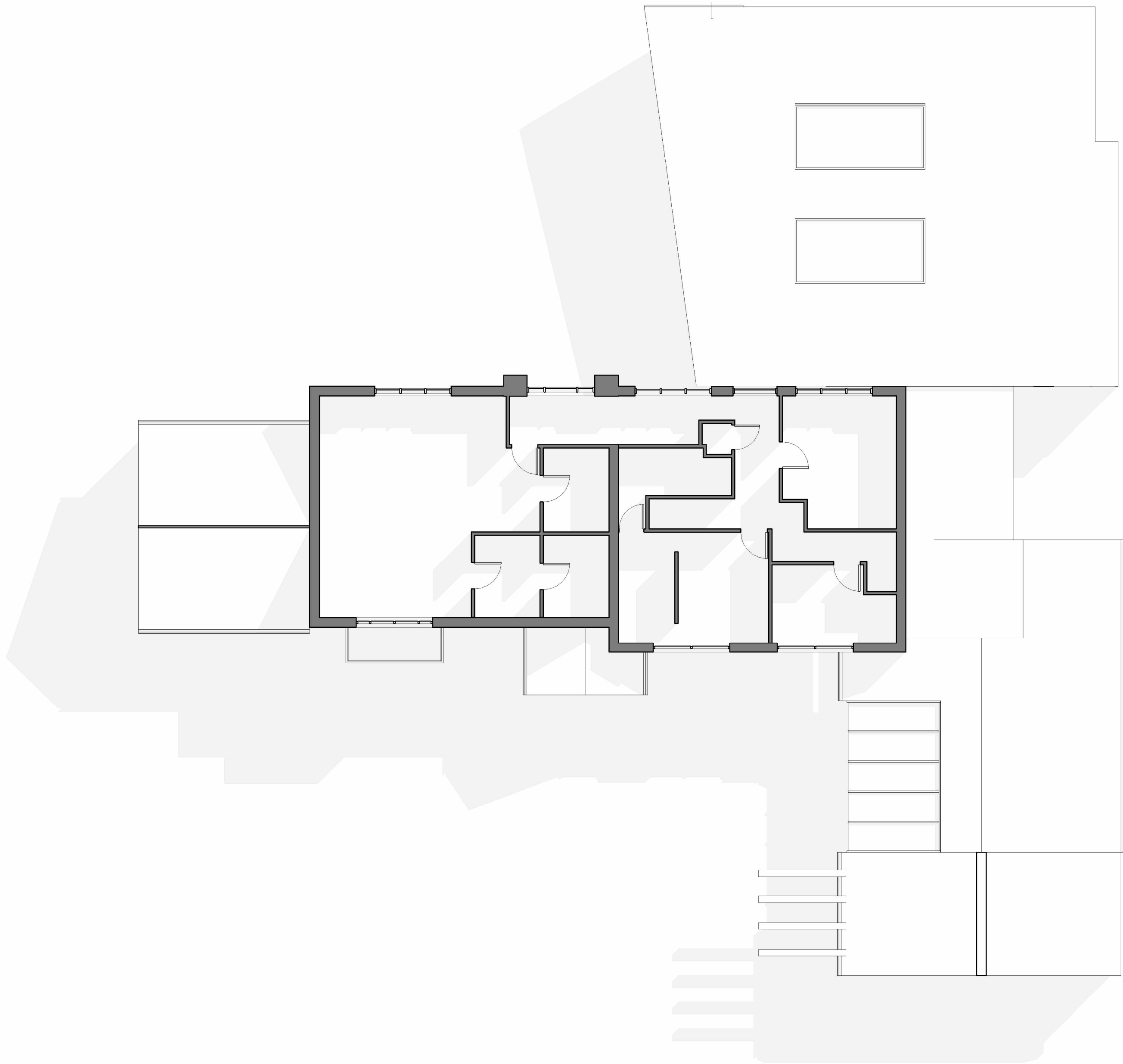
2 Proposed First Floor 1 : 100
