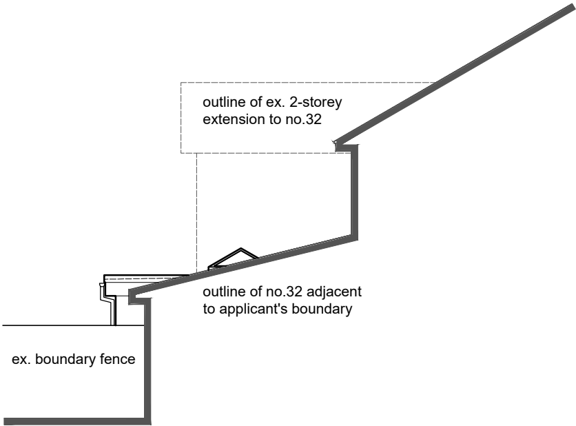
SIDE ELEVATION (facing onto 32 Bagslate Moor Road)
