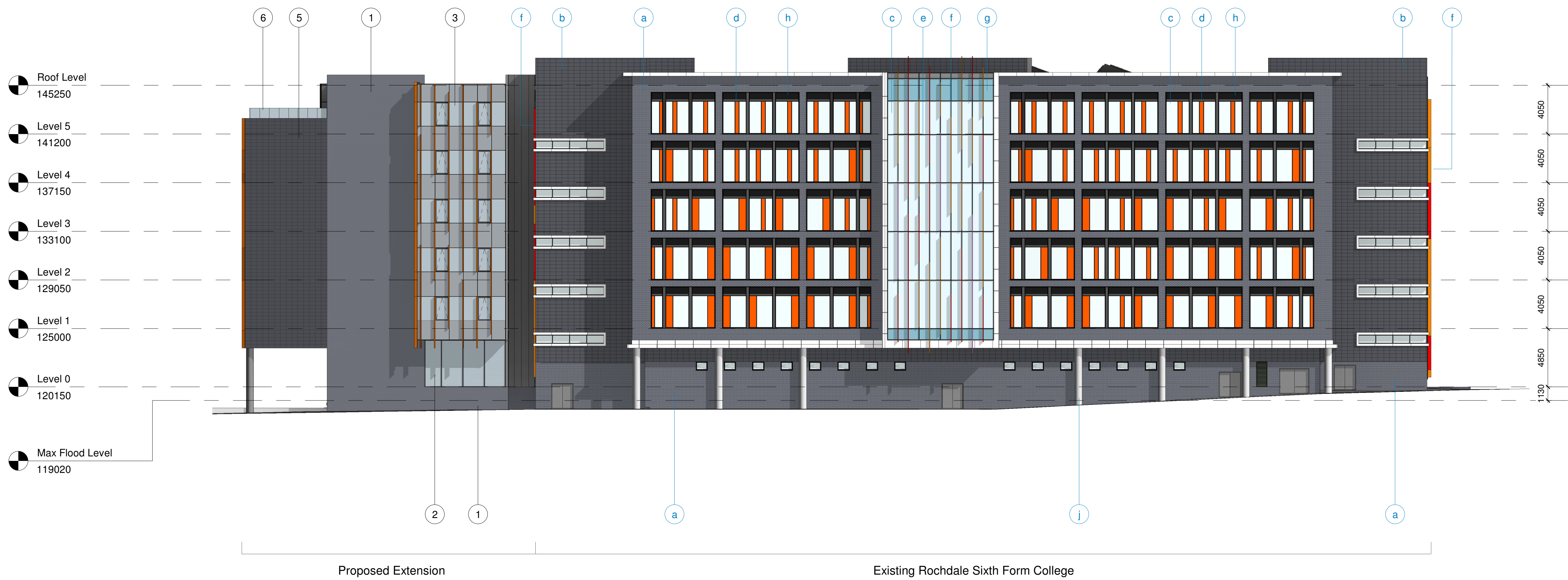
GA Elevation - South West 1 : 200
