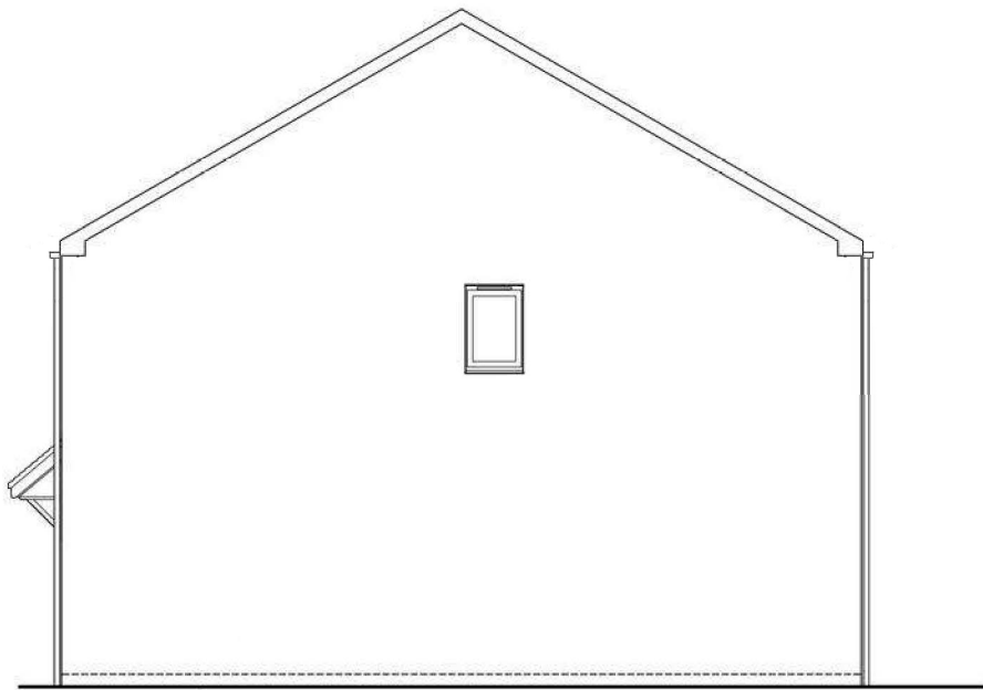
SIDE ELEVATION END/SEMI DETACHED EMA33 (2B4P)
