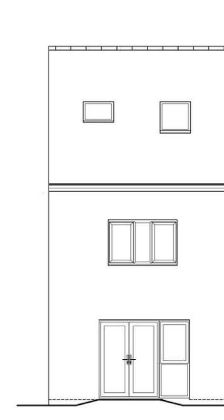
REAR ELEVATION END/SEMI DETACHED EMB3 I (3B5P)
