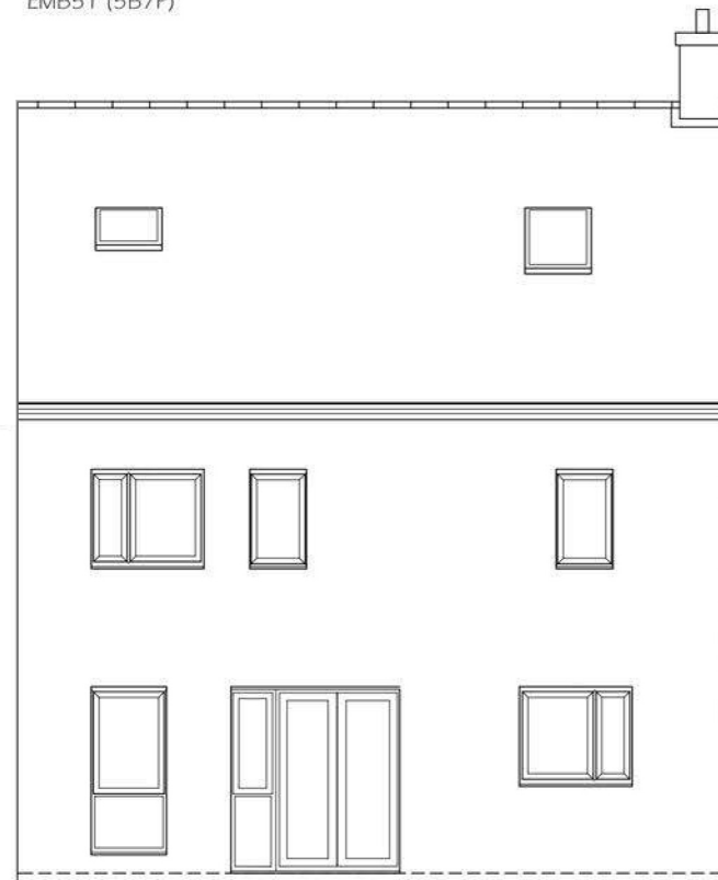
REAR ELEVATION DETACHED EMB5 I (5B7P)
