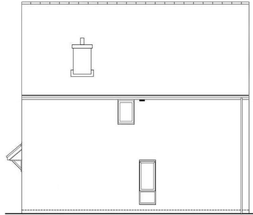
SIDE (RIGHT) ELEVATION DETACHED EMA43 (4B5P)
