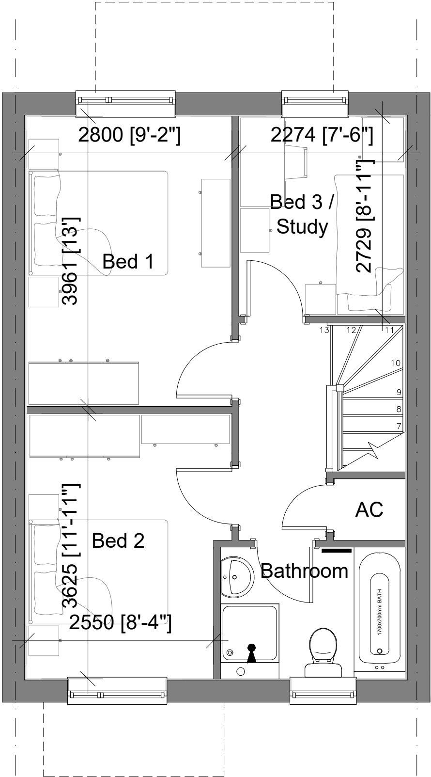
First Floor
