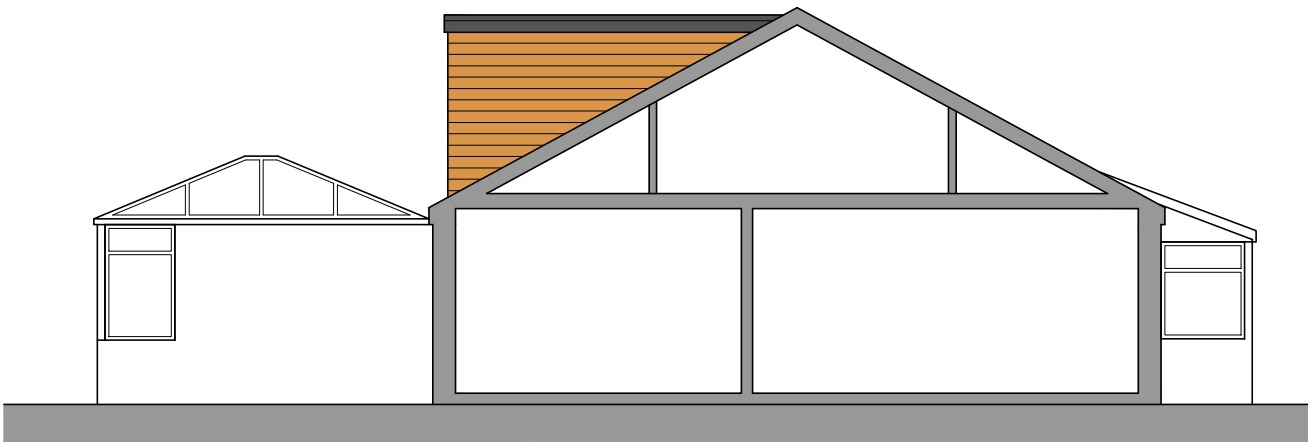
West Facing Side Elevational Section
