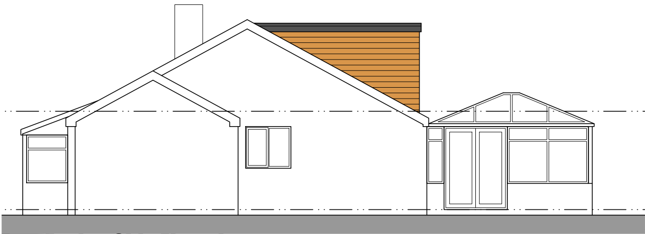
East Facing Side Elevation
