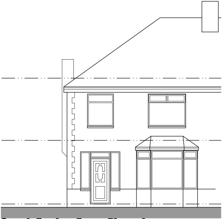
South Facing Front Elevation
