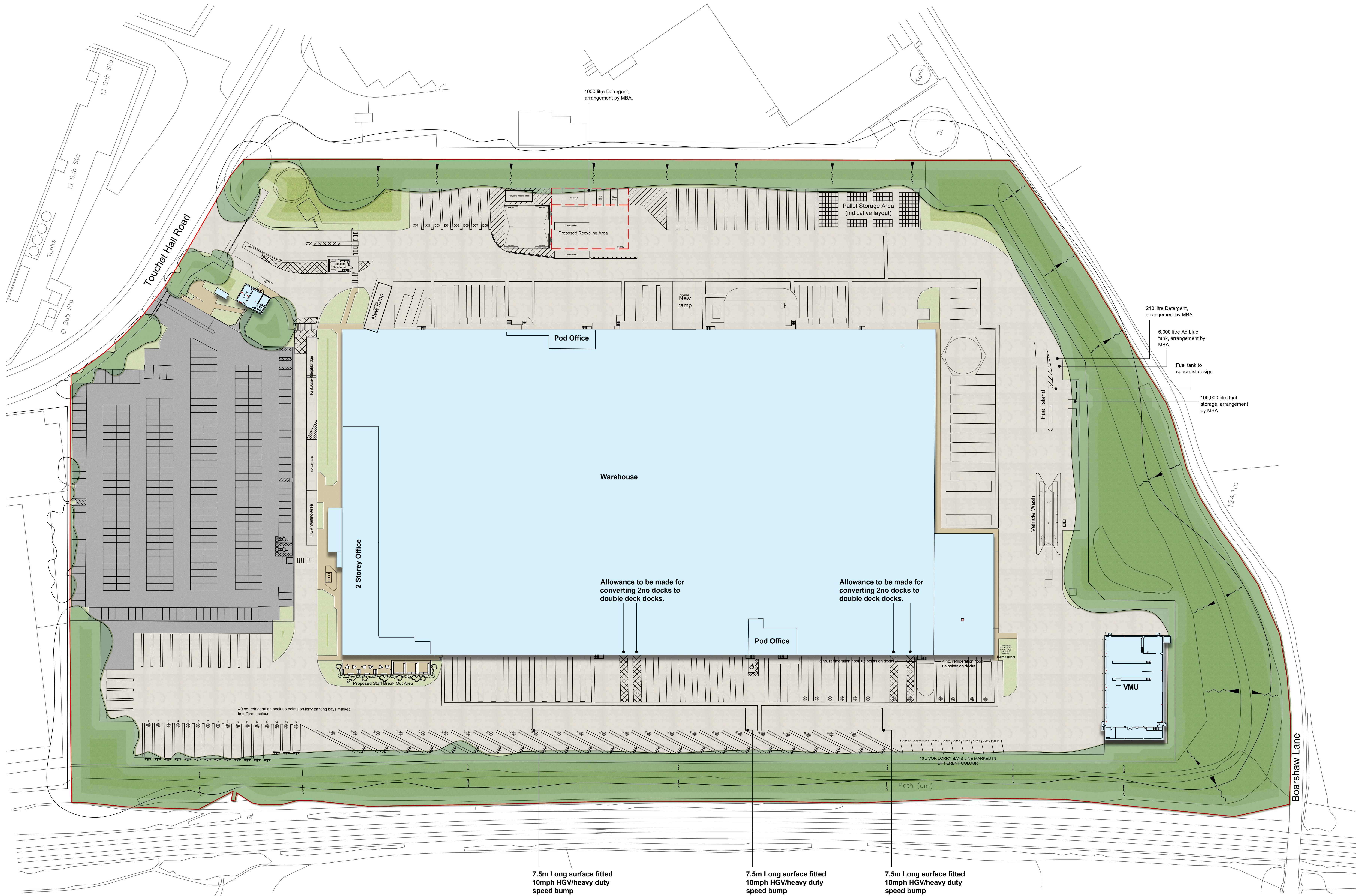
Proposed Site Layout Scale 1:500
