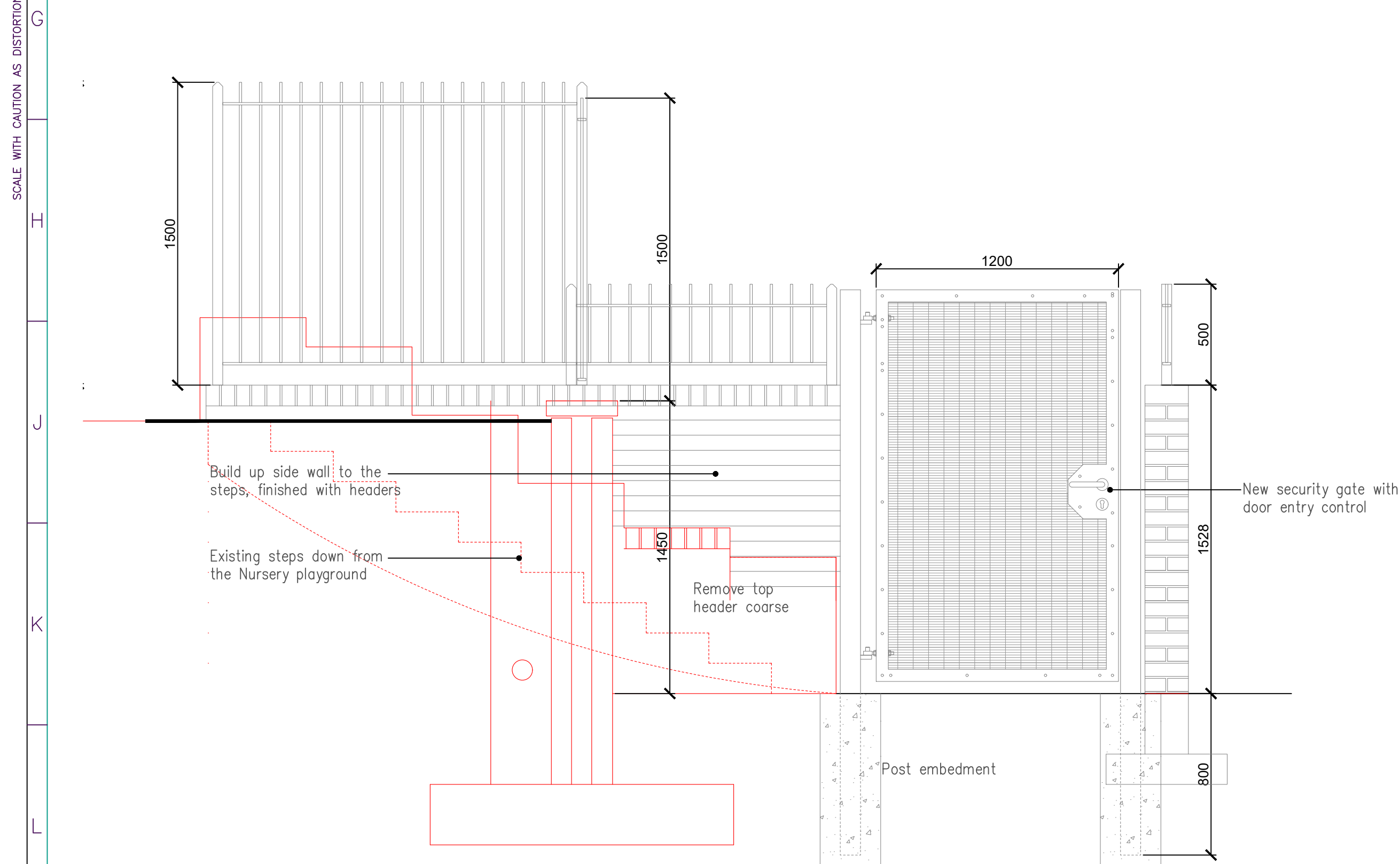
SIDE ELEVATIONS TO THE STEPS ENCLOSURE AREA Scale 1:20
