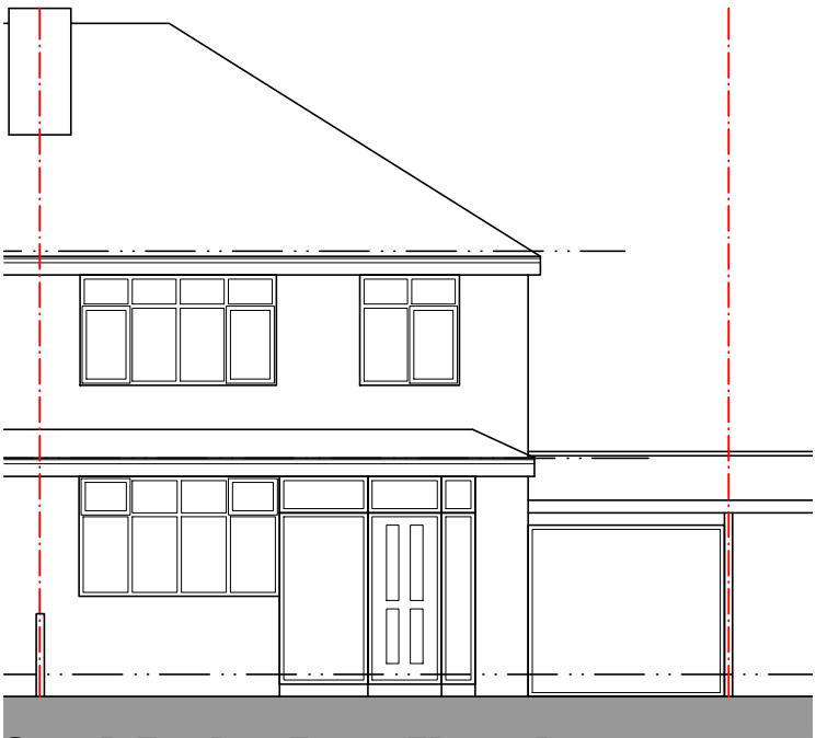
South Facing Front Elevation
