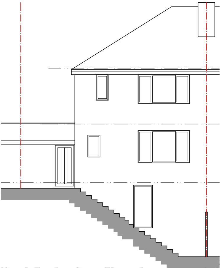
North Facing Rear Elevation
