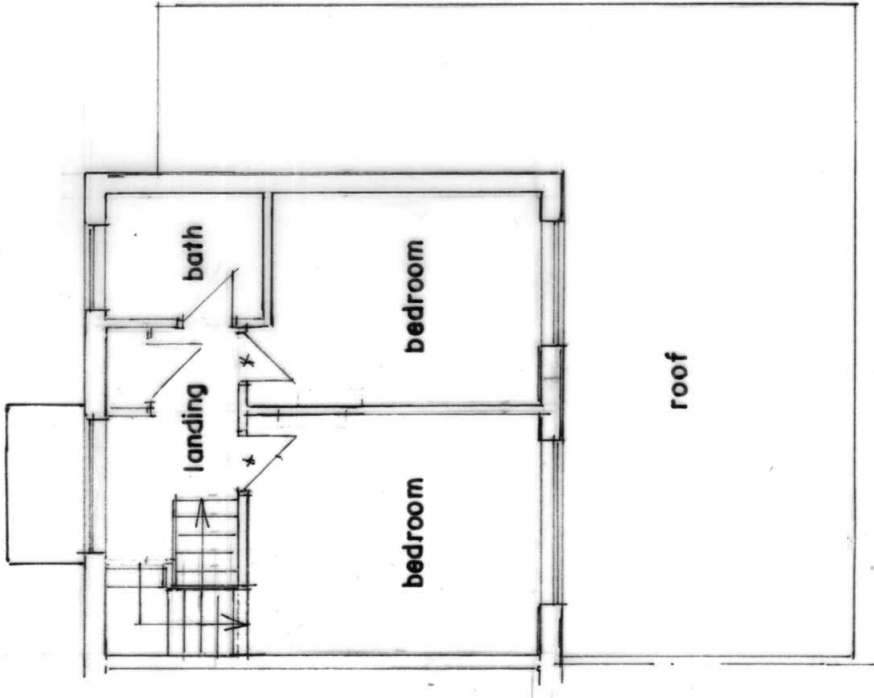
FIRST FLOOR PLAN (PROPOSED)
