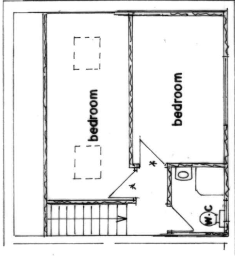
SECOND FLOOR PLAN (PROPOSED)
