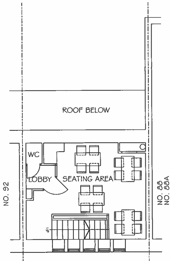
EXISTING FIRST FLOOR 1:100 LAYOUT
