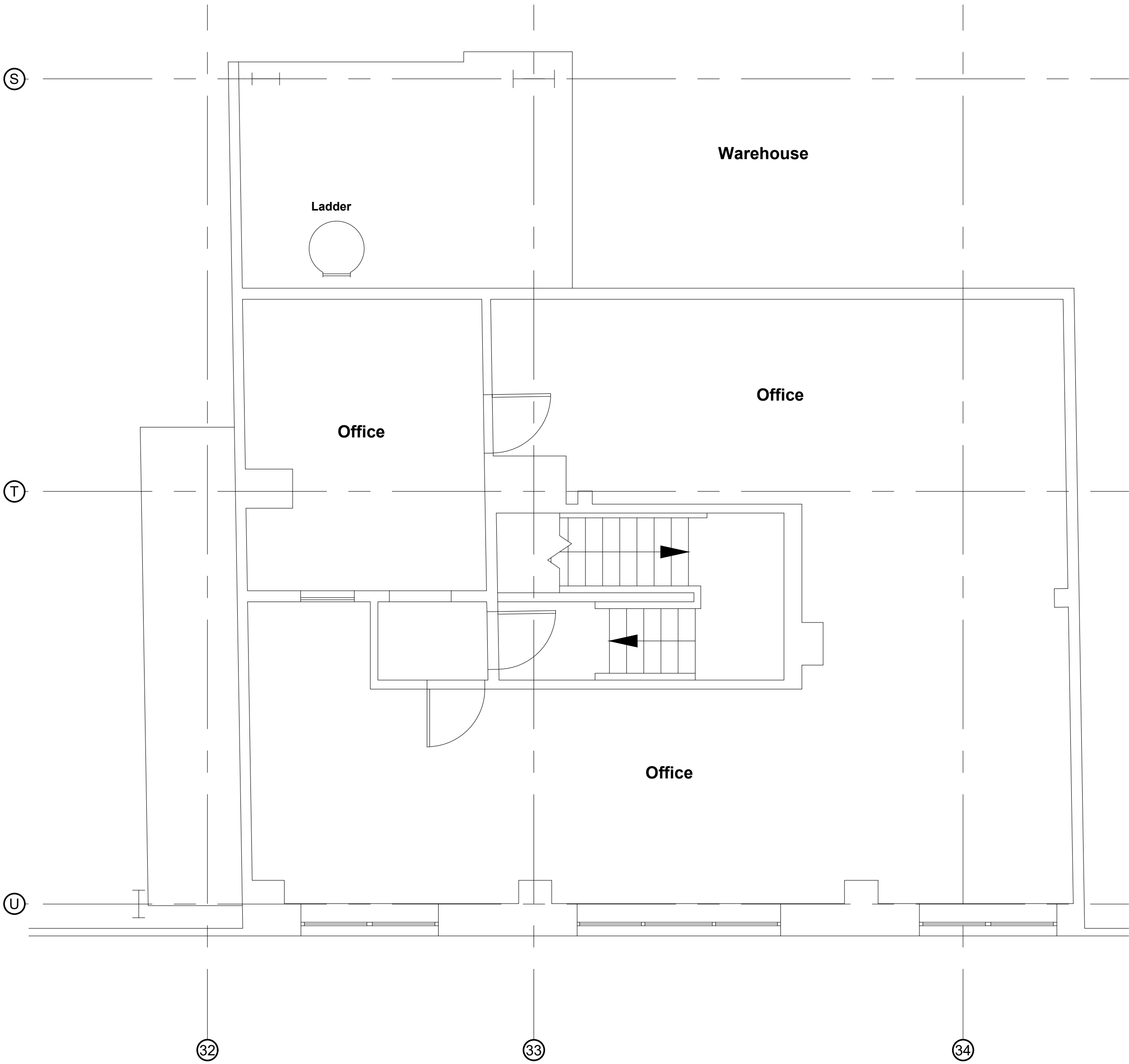
Existing Pod Office - First Floor Scale 1:50
