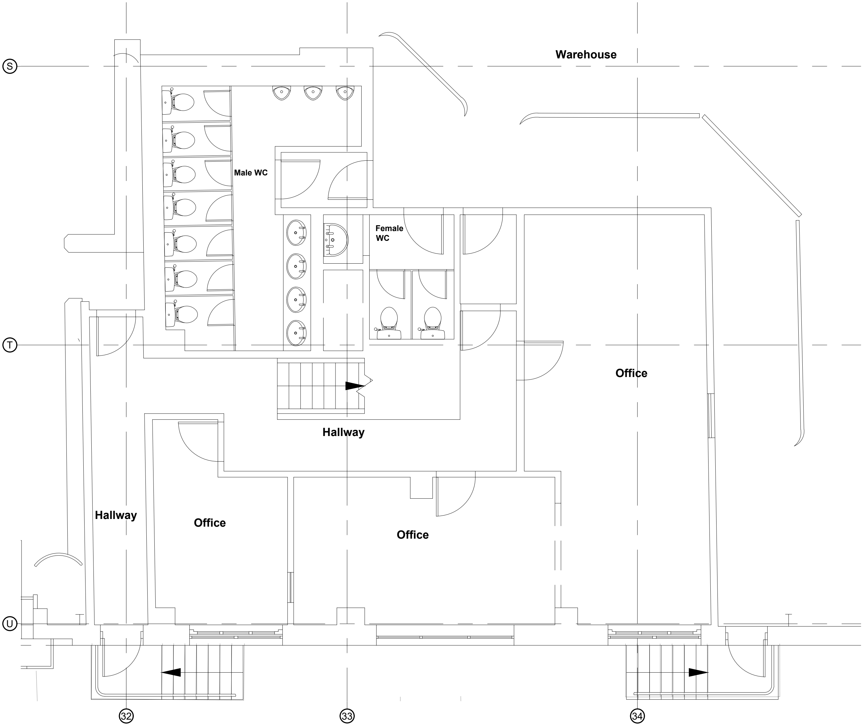
Existing Pod Office - Ground Floor Scale 1:50
