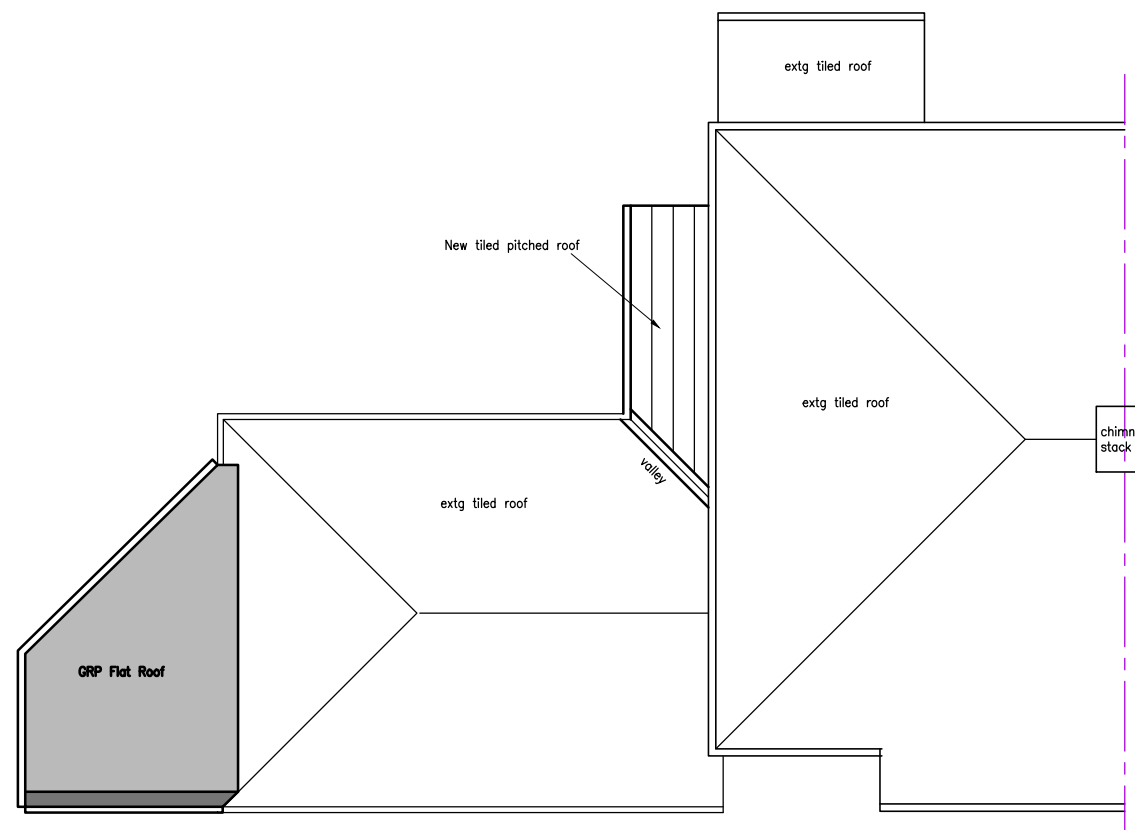
ROOF PLAN
