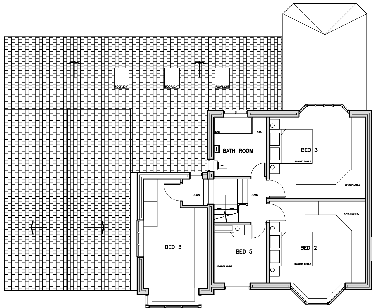
PROPOSED FIRST FLOOR LEVEL
