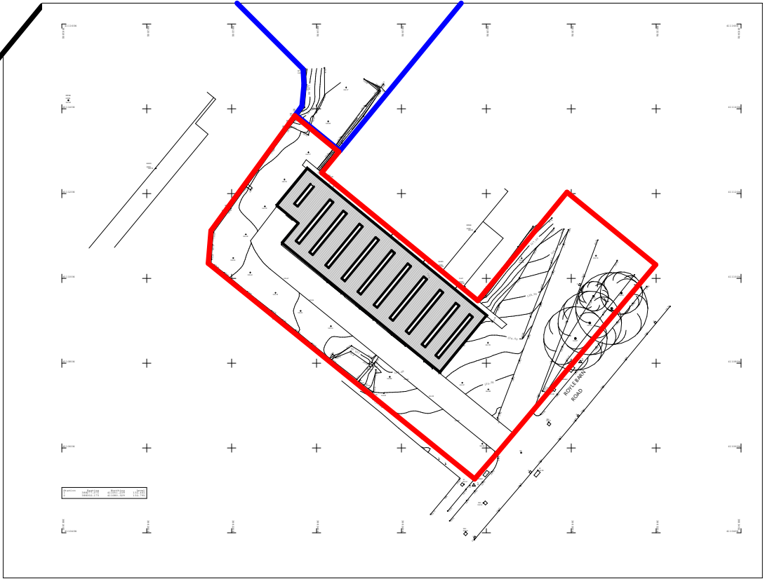
2 Proposed Location Plan 1 : 1250
