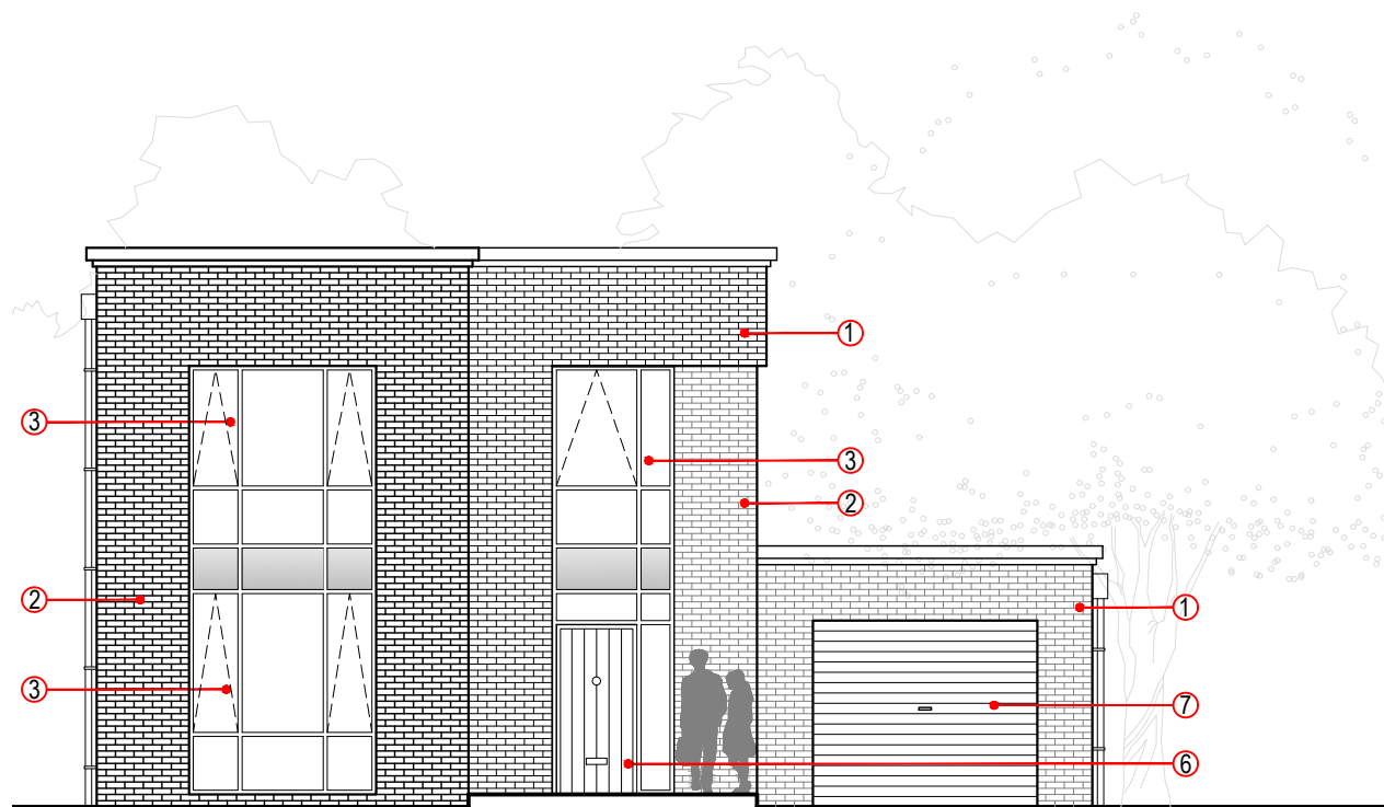
PROPOSED FRONT ELEVATION 1:100@A3
