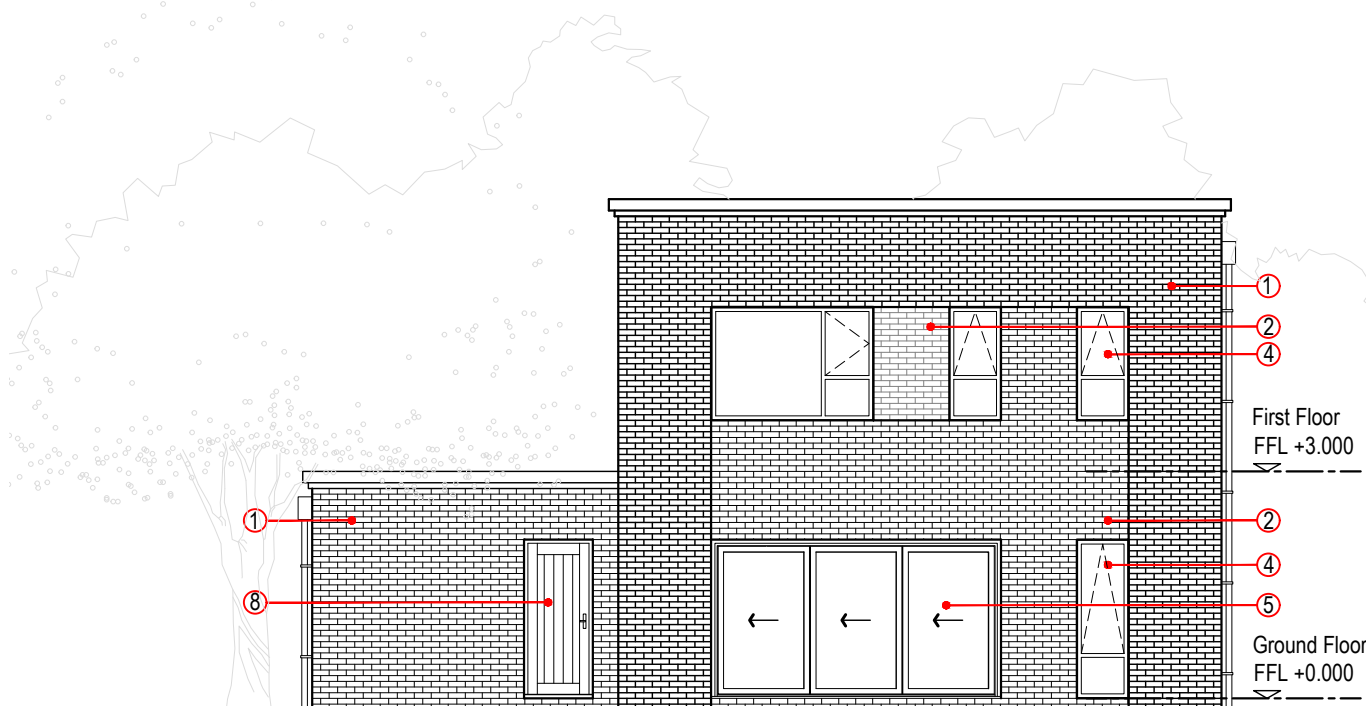
PROPOSED REAR ELEVATION 1:100@A3
