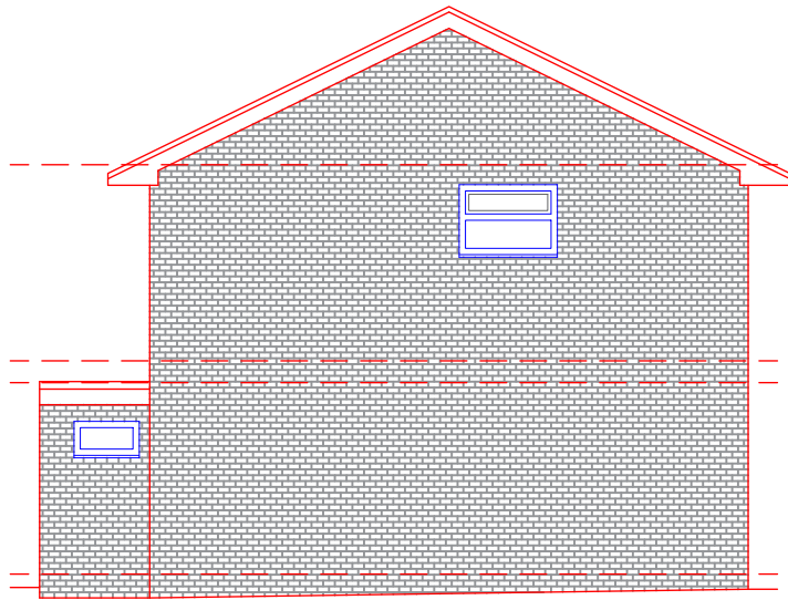
Existing Side Elevation 1 @1:100
