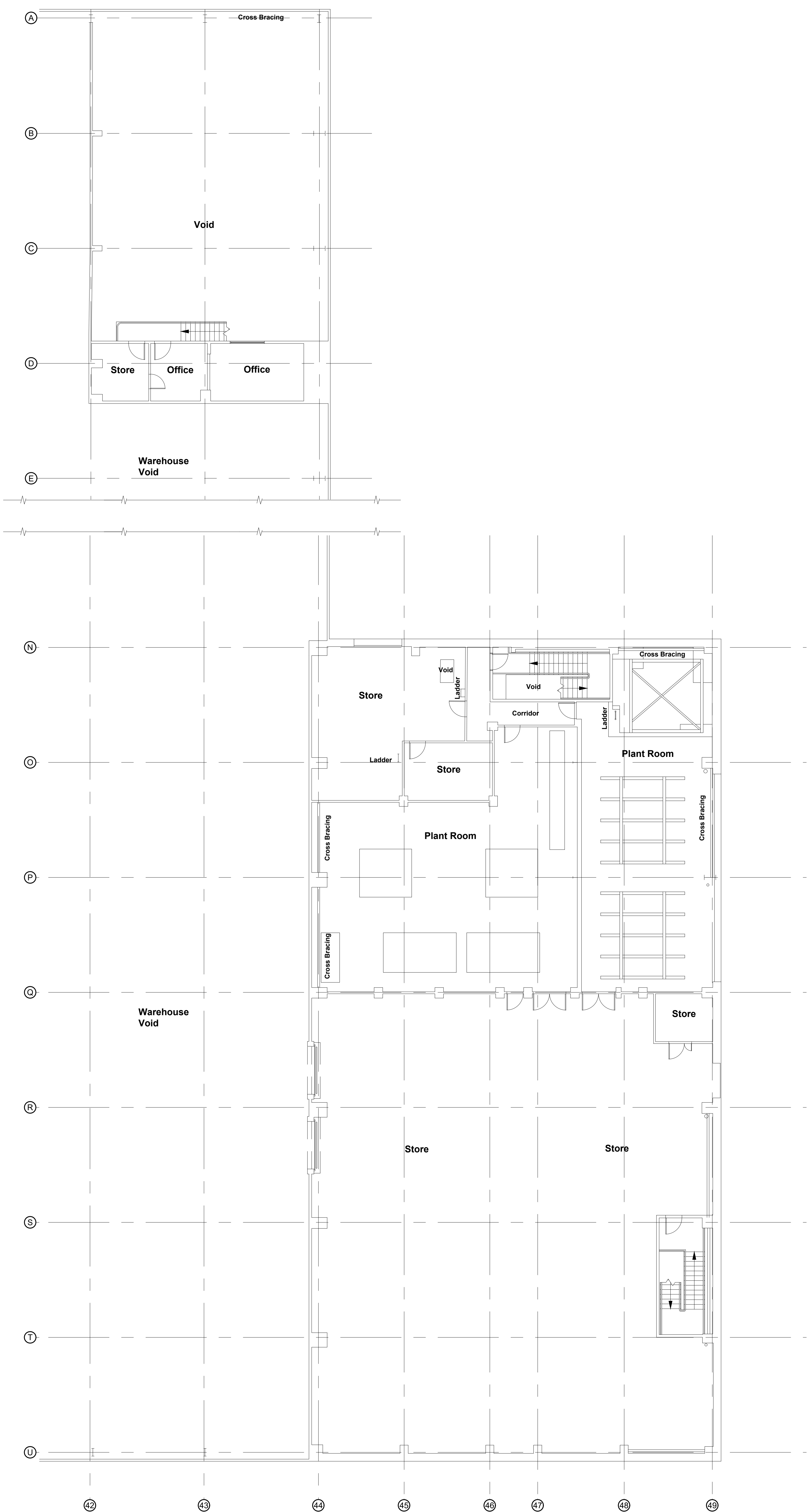
Existing South Store - First Floor Scale 1:100
