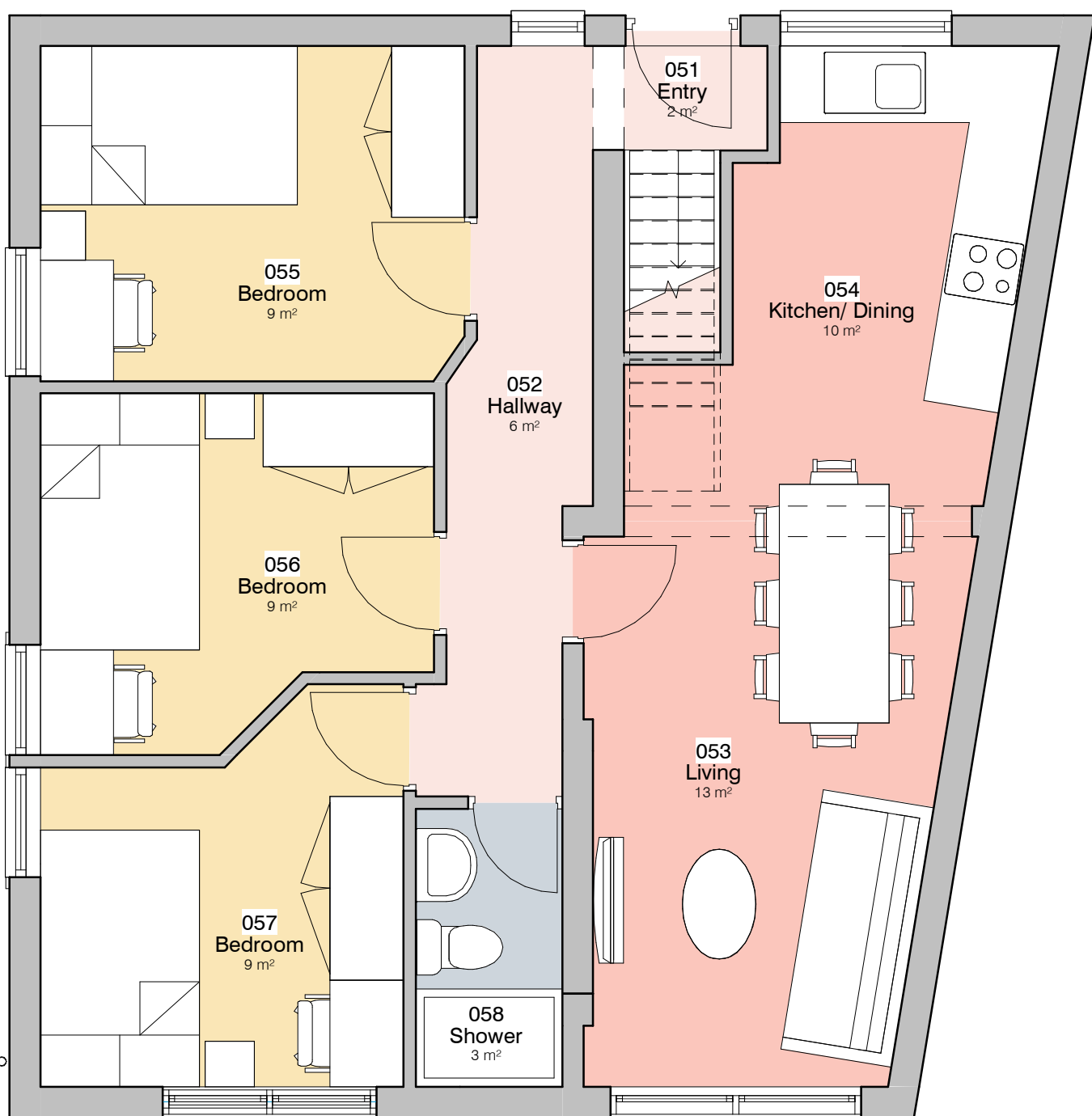
5. Level 0 - GA Proposed 1:50
