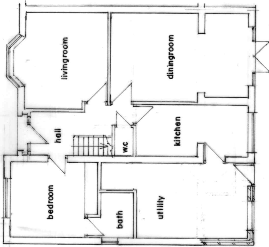
GROUND FLOOR PLAN (PROPOSED)
