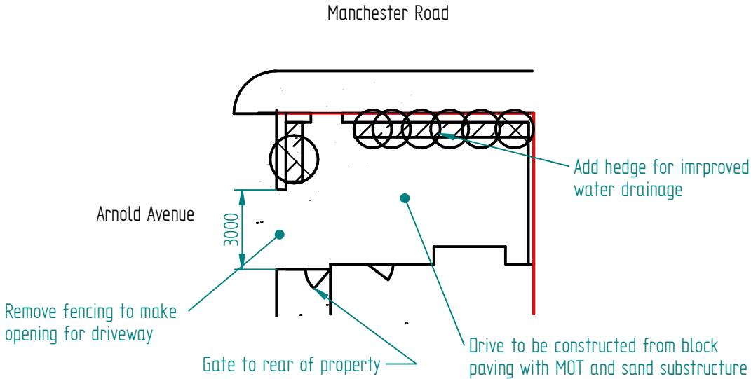
2. Proposed Site 1 : 200
