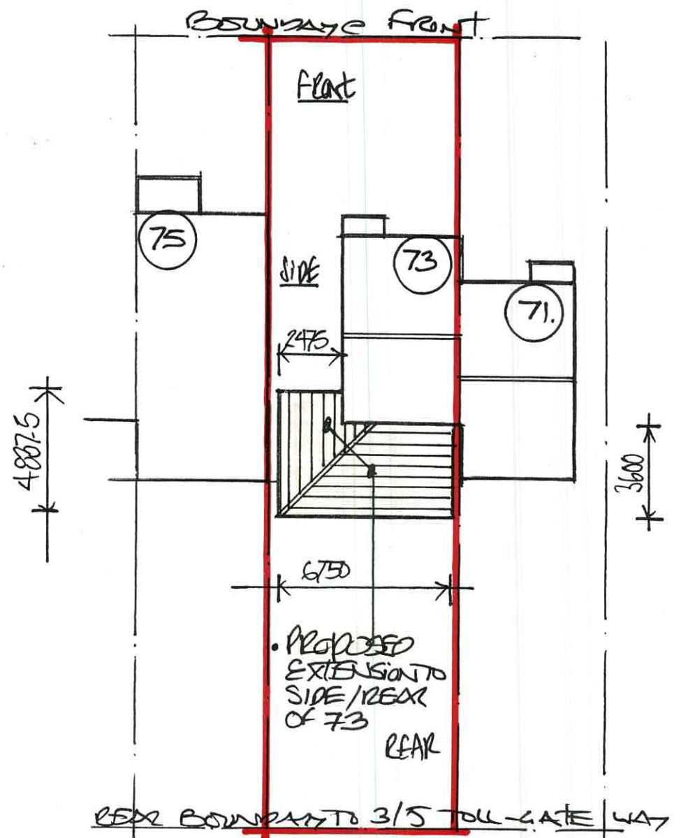
1:200 'PROPOSED' BLOCK PLAN
