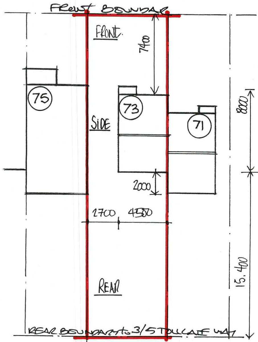
1:200 EXISTING 'BLOCK PLAN'
