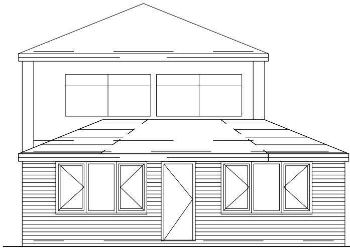
FRONT ELEVATION (PROPOSED)
