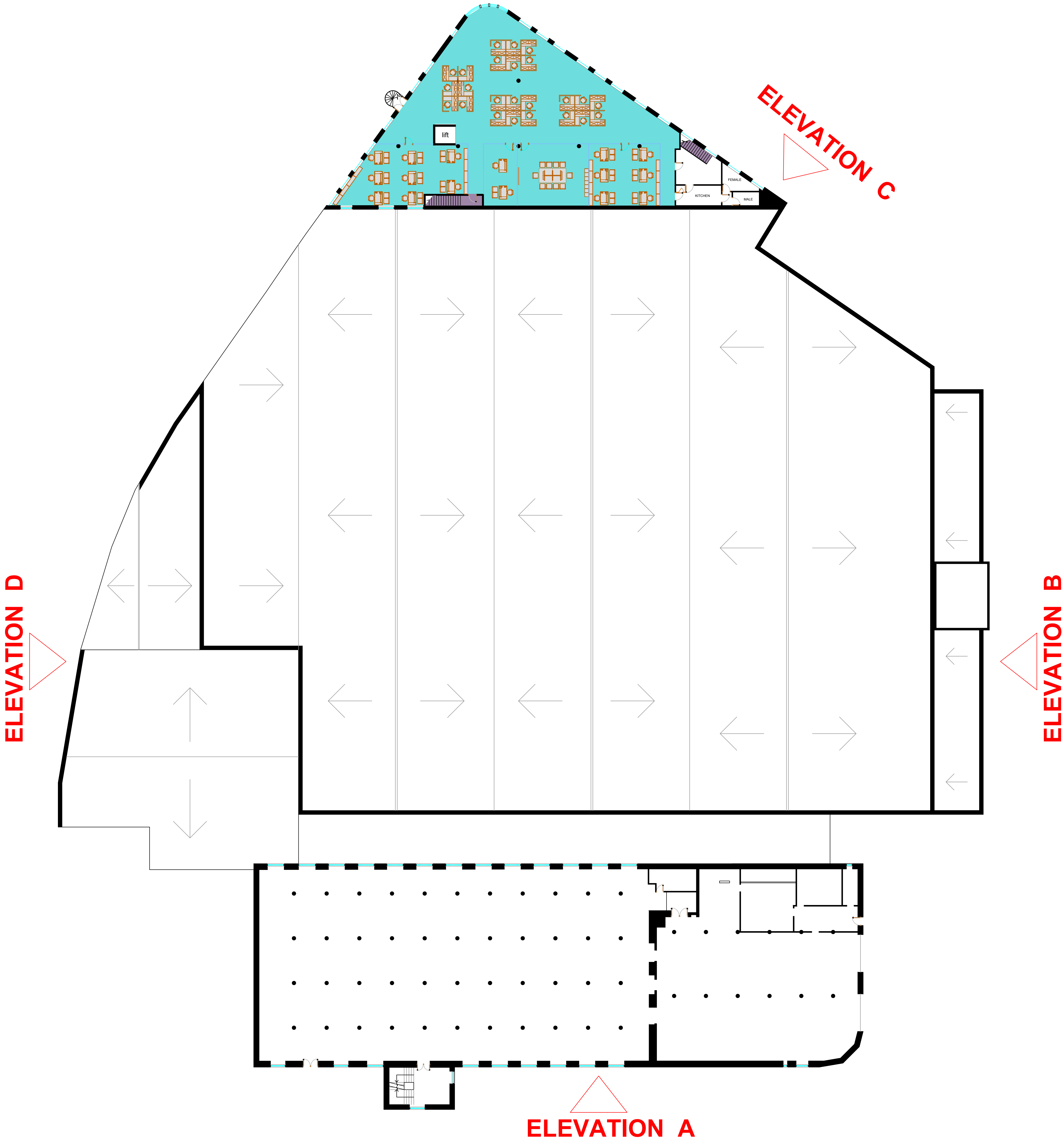
PROPOSED GROUND FLOOR PLAN 1:500 @ A0
