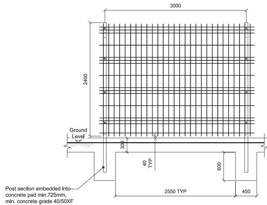
TYPICAL 2.4m GREEN WELDMESH FENCE DETAIL
