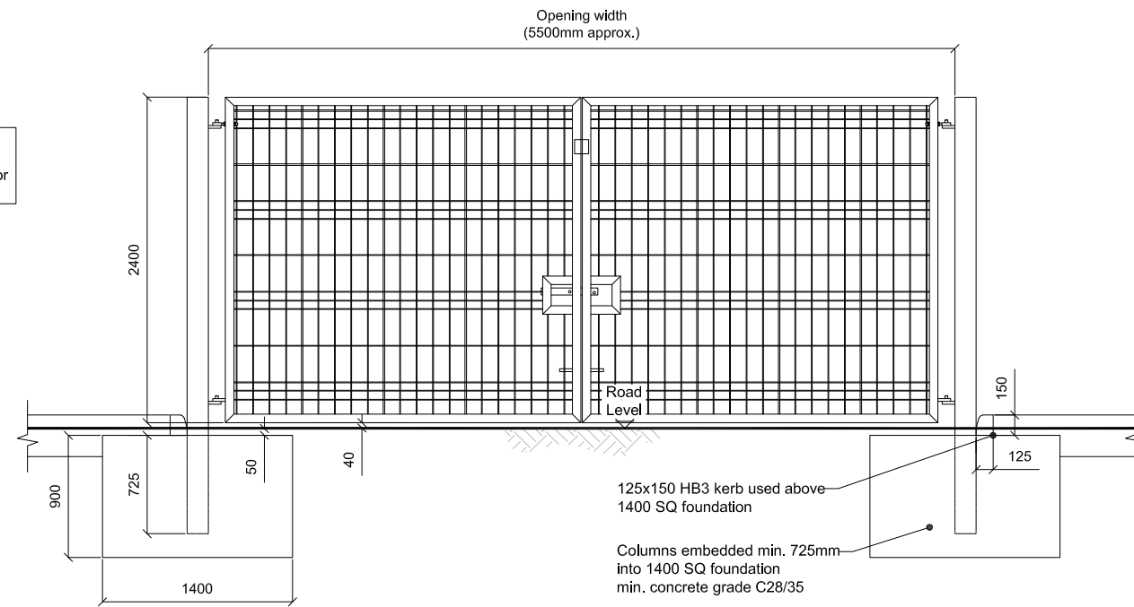
TYPICAL 2.4m GREEN WELDMESH GATE DETAIL
