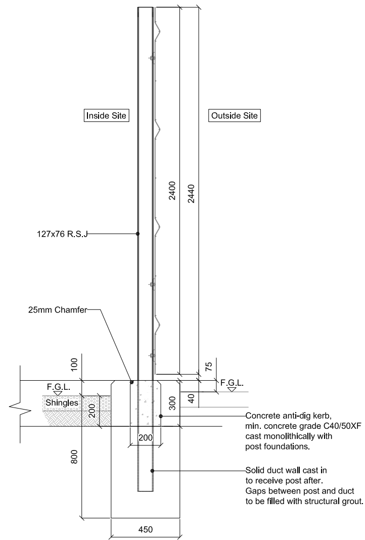
TYPICAL FENCE SECTION DETAIL
