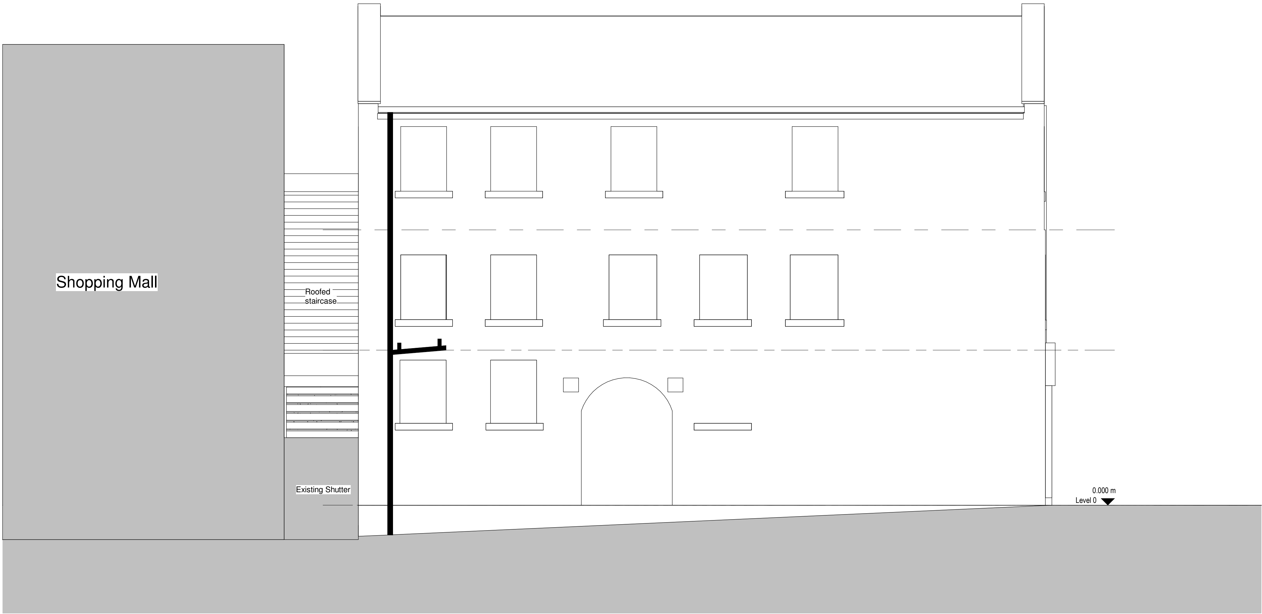
1 Existing Side Elevation 1 : 50
