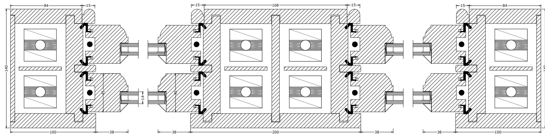
Sash Window With Mullion Horizontal Section Detail
