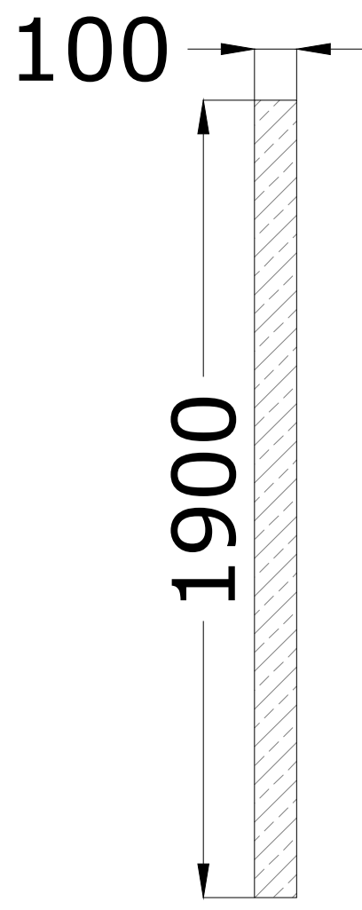
Proposed Continuous Sand Stone Jamb for DR01. X2
