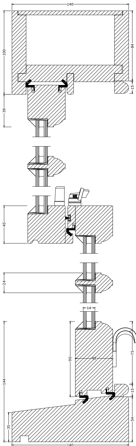
Sash Window Vertical Section Detail
