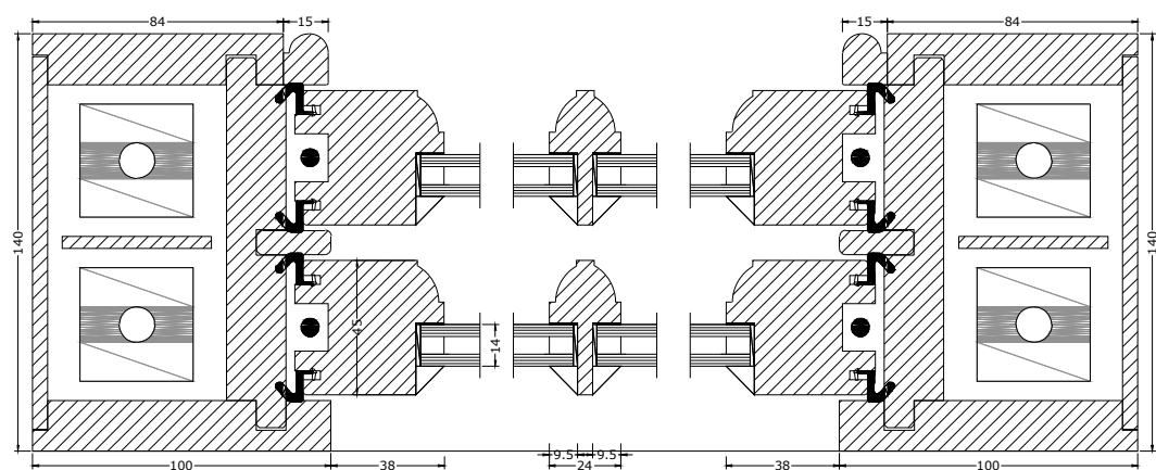
Sash Window Horizontal Section Detail
