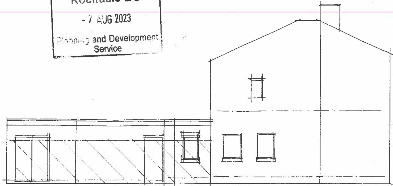
ELEVATIONS SIDE 1:100
