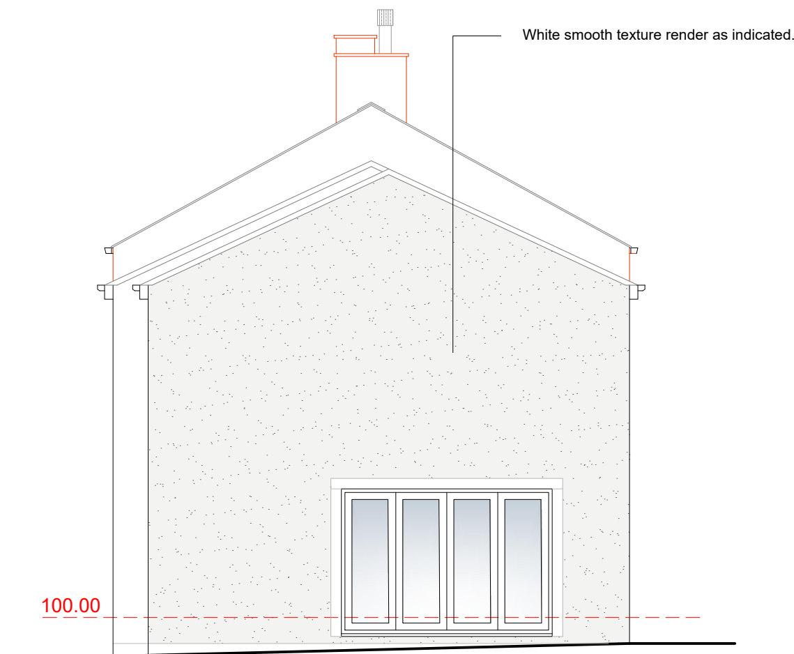
PROPOSED SIDE ELEVATION 1
