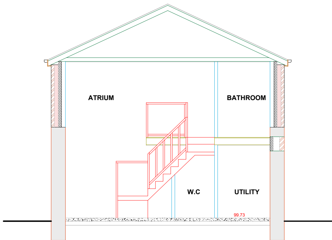
PROPOSED SIDE ELEVATION 1
