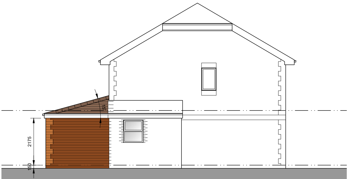
East Facing Side Elevation
