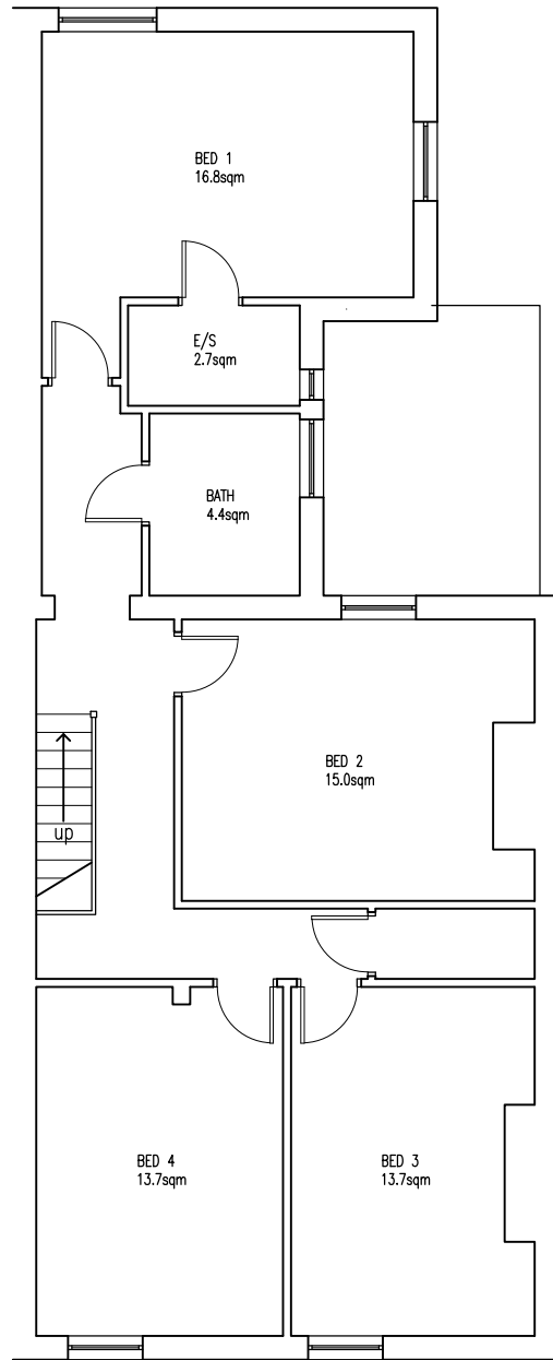
EXISTING FIRST FLOOR PLAN 1:100 @ A3
