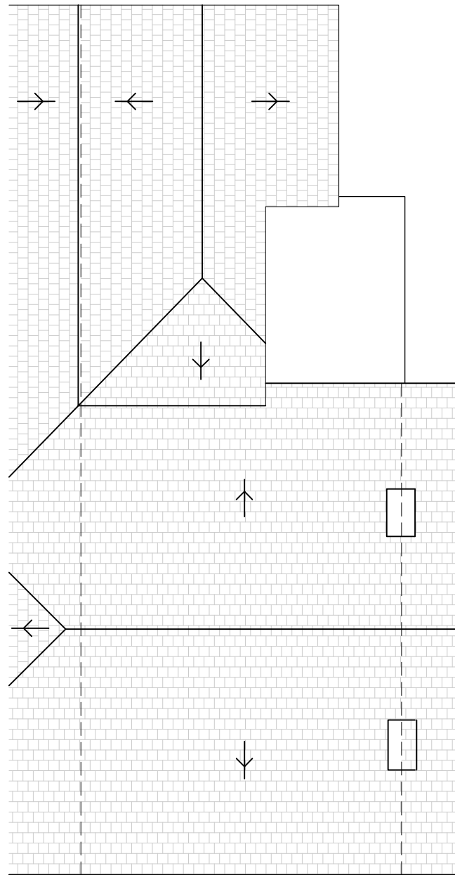
EXISTING ROOF PLAN 1:100 @ A3
