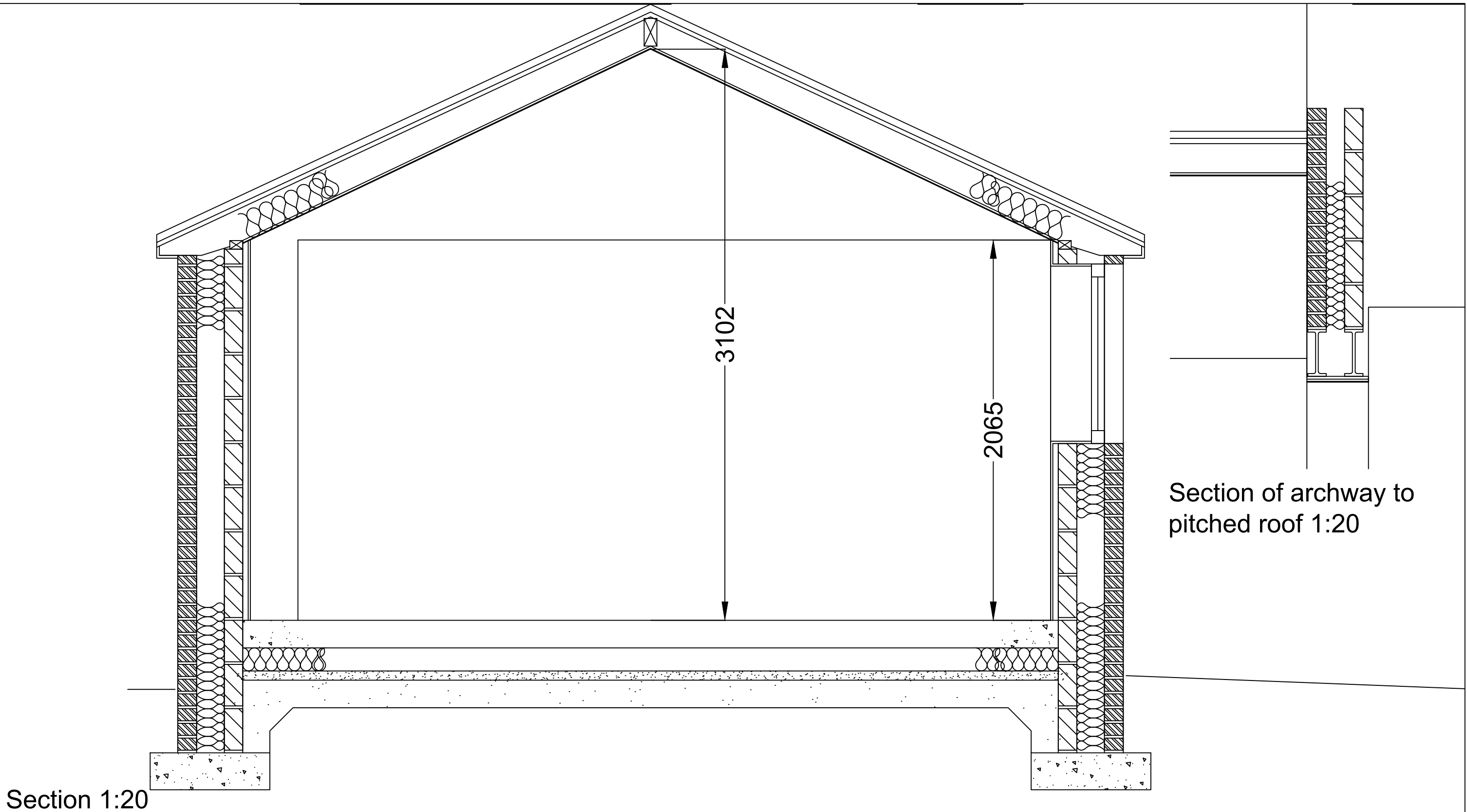
Section 1:20
