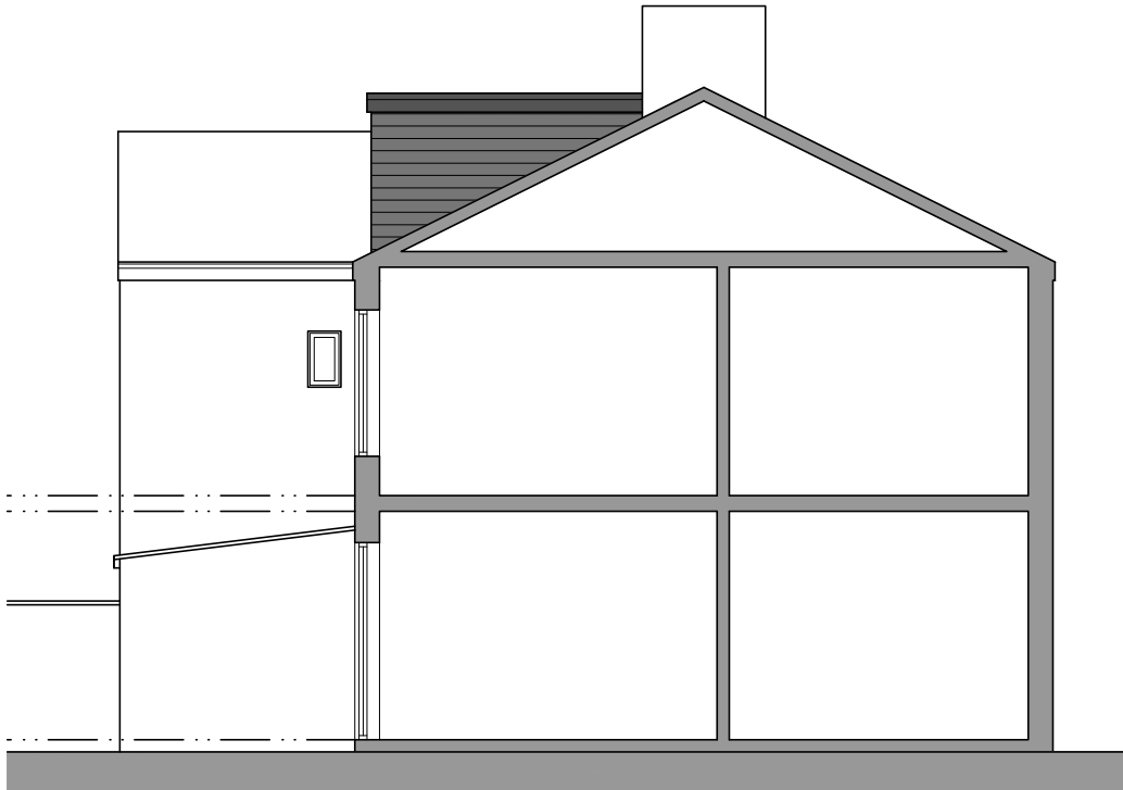
West Facing Side Elevation
