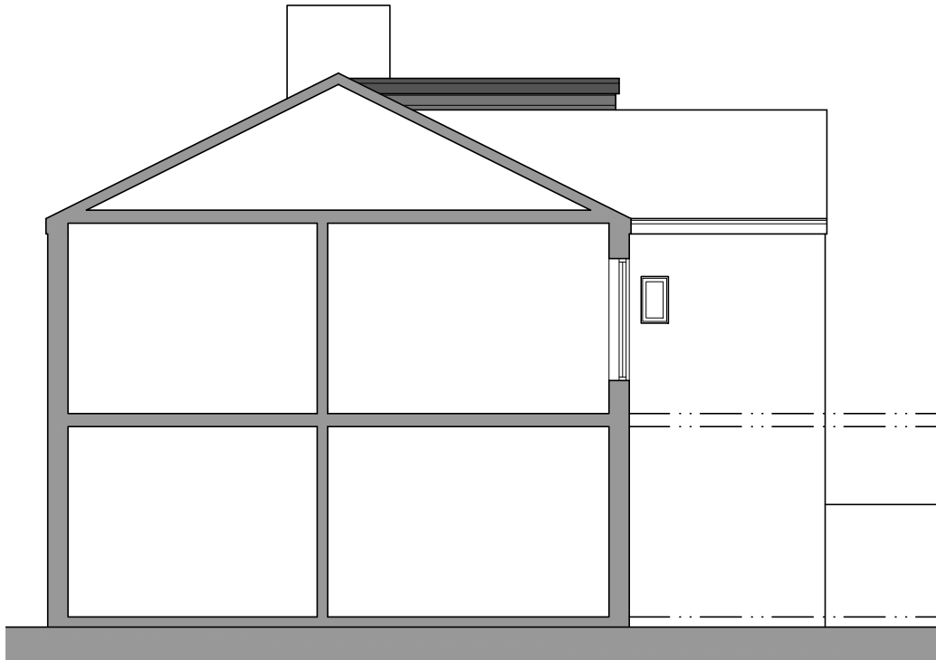
East Facing Side Elevation
