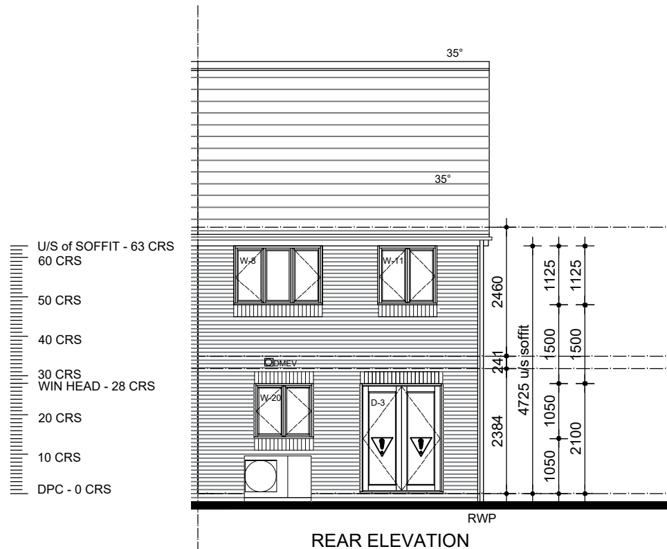
REAR ELEVATION
