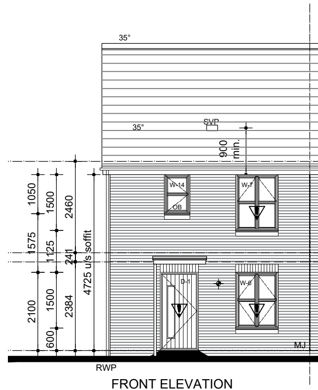
FRONT ELEVATION
