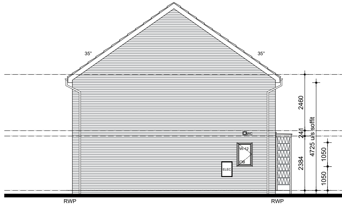
SIDE ELEVATION
