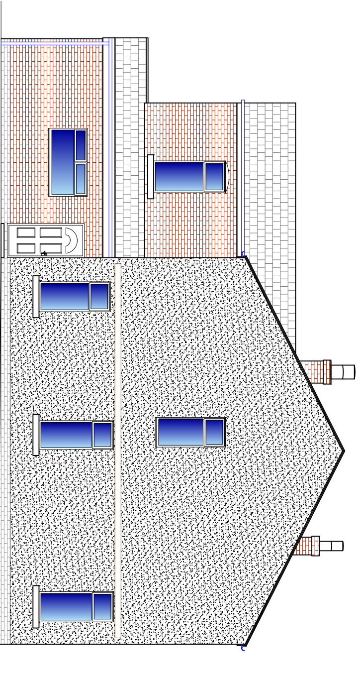
Existing Side Elevation 1:100
